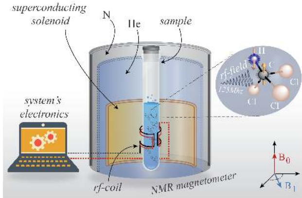
Figure 2. (Color online) We show a section of the magnetometer employed in our NMR experiment. A superconducting magnet, which produces a high intensity magnetic field ( B_0 ) in the longitudinal direction, is immersed in liquid He, surrounded by liquid N in another vacuum separated chamber, in a thermally shielded vessel. The liquid sample (inside a 5mm glass tube) is placed at the center of the magnet within the rf-coil of the probe head. A digital electronic time-modulated-pulse induces a transverse rf-field ( B_1 ) that drives the ^{13}\text{C} nuclear spins out of equilibrium. In the forward (backward) protocol, the rf-coil can perform (can retrieve) work on (produced by) the nuclear spin sample. Depending on the speed of the modulation of the driving field, irreversible entropy is produced. The sketch is not in scale and has been stripped of unnecessary technical details of the apparatus.
