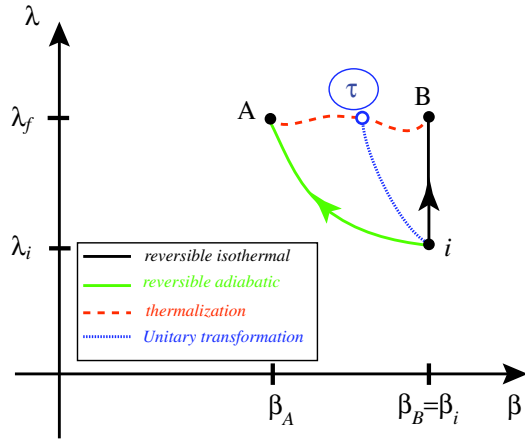
FIG. 1 (color online). Sketch of the transformations considered. The full black circles represent equilibrium states \rho_i = Z_i^{-1} e^{-\beta_i H_i} , \rho_A = Z_A^{-1} e^{-\beta_A H_f} , and \rho_B = Z_B^{-1} e^{-\beta_B H_f} . The empty blue one, instead, is the state at time \tau , \rho_\tau = U(\tau, 0)\rho_i U^\dagger(\tau, 0) .
