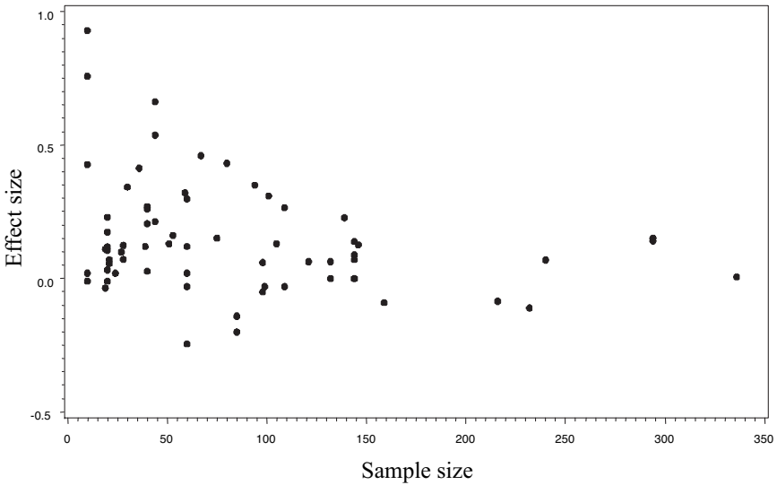
FIGURE 2 Funnel plot of effect sizes (in z) for actual similarity against sample size, field studies only
