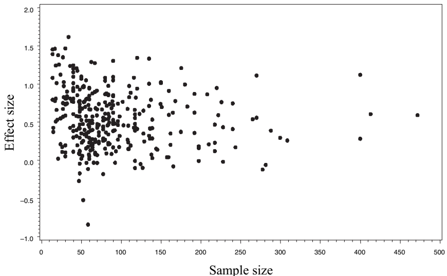
FIGURE 1 Funnel plot of effect sizes (in z ) for actual similarity against sample size, laboratory studies only
