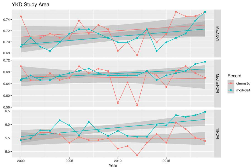
FIG. 4. Time series intercomparison of the regional average (top) MaxNDVI, (middle) MedianNDVI, and (bottom) TI-NDVI for GIMMS and MODIS. Time series are not shown for Landsat sensors because of excessive data gaps.
