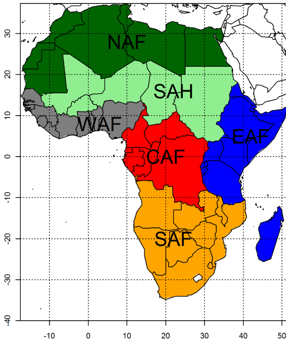
Figure S1 Zone typology in the African continent as used in the study, designed to match with the study of Lobell et al. (Lobell et al., 2008)
