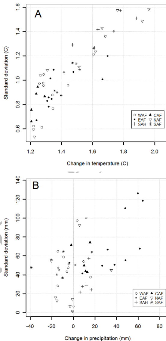
Figure 1 Predicted changes in climates as averages of 24 GCMs (Table 2) and uncertainties expressed as standard deviations of the GCMs. (A) Annual mean temperature, (B) total annual rainfall. Zone typology as in Figure S1.
