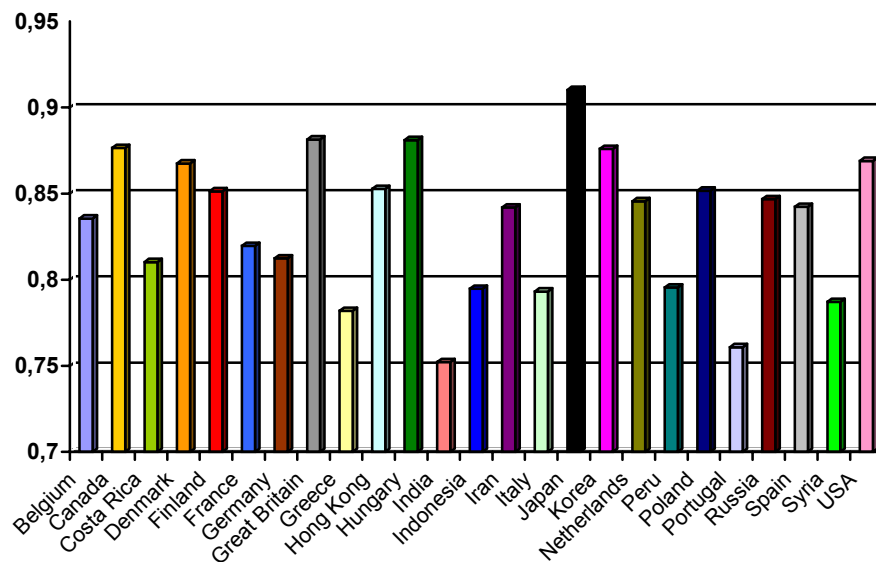
Figure 1: Scale reliabilities (Cronbach's Alpha) for all nations
