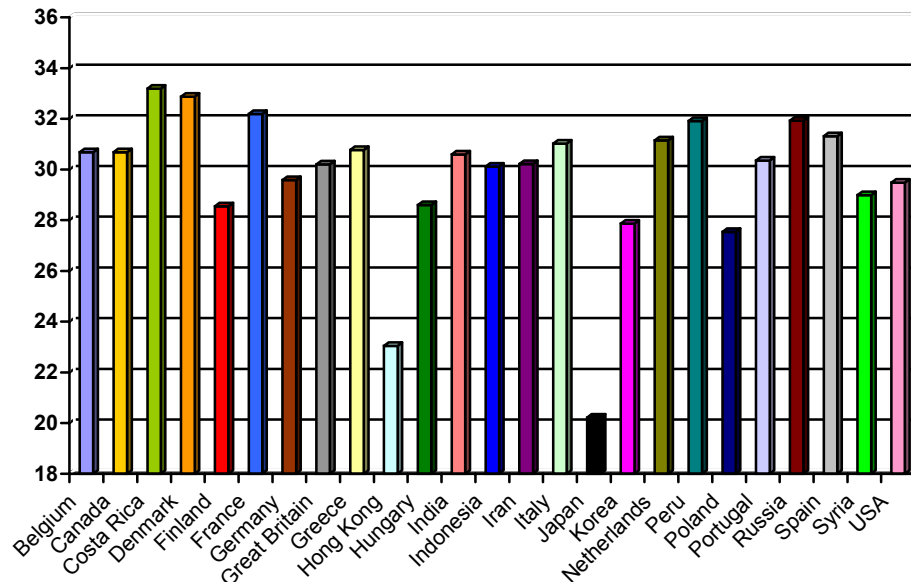
Figure 3: Mean sum scores broken down by nation.
