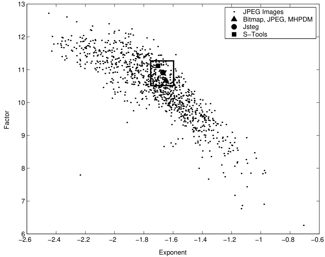
Figure 2: Cloud of Areas Model parameters values for JPEG images and the effect of hiding information on one particular image. Note that the variation due to the hiding process is rather small compared to the intrinsic variability of the parameters for this class of natural images.
