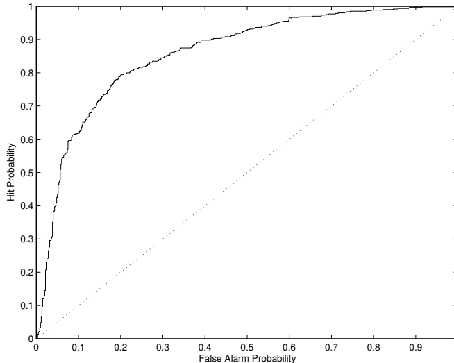
Figure 10: Results using Coefficients Correlations Estimation. The graph shows that this technique, that uses information about the stego algorithm, can detect stego images with significant accuracy.
