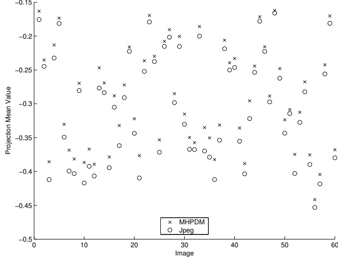
Figure 9: Projection of DCT coefficients. Although the values are similar for the natural and stego images, there is a clear bias, being the value for the stego image always greater than the one for the corresponding natural one.
