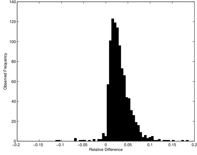
Figure 5: Histogram of relative differences between parameter p of PC Model for a MHPDM image and its corresponding JPEG image. We observe that values of relative differences (difference divided by the value of p for JPEG image) are mostly smaller than 5% and practically all values are positive.
