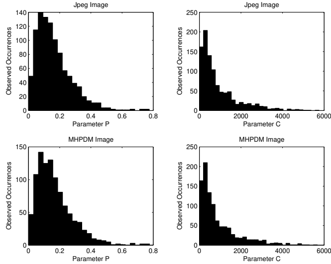
Figure 6: Histograms of PC Model parameters for JPEG and MHPDM images. We observe that the parameters distributions are similar for natural and stego images.
