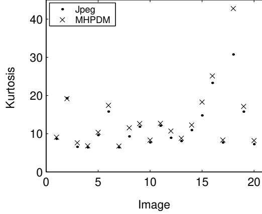
Figure 8: Estimated kurtosis of differences of adjacent horizontal Haar wavelet coefficients. We observe a clear bias in the stego image.
