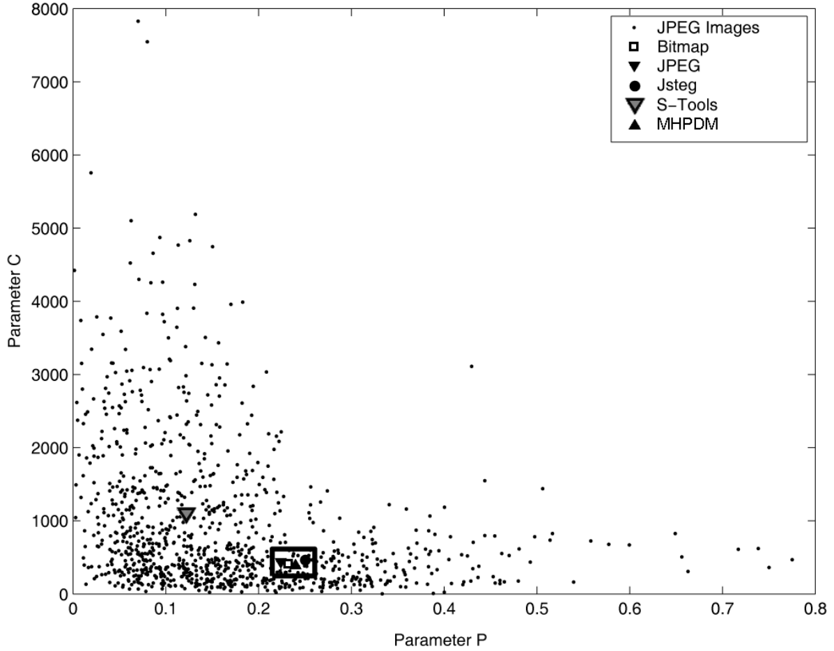
Figure 4: Cloud of PC Model parameters values for JPEG images and the effect of hiding information on one particular image. Enclosed in a frame are values for bitmap, JPEG, Jsteg and MHPDM versions of the same image. The value for the same image processed with S-Tools, outside the frame, clearly shows that S-Tools produces easy to detect non-natural images (following this model), while MHPDM and Jsteg do produce what are considered legitimate natural images.
