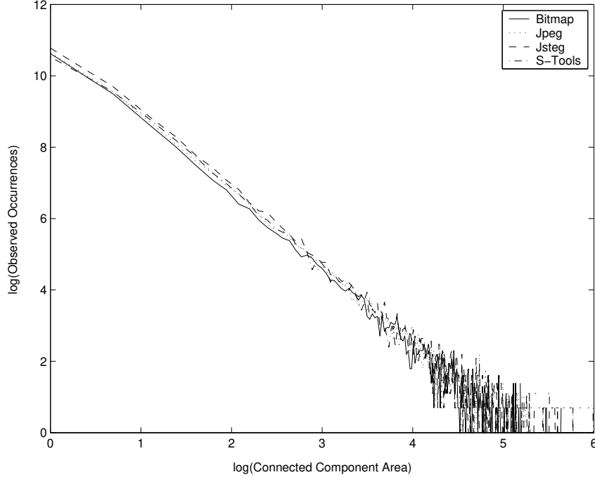
Figure 1: Distribution of connected components areas for four versions of the same image, with and without hidden message. We observe that the exponential distribution is observed both by the original and the stego images, thereby limiting the use of this model for stego-analysis.
