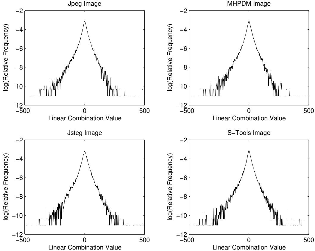
Figure 7: Parameter distribution for the Differentially Laplacian Model for the four classes of images. We observe very similar distributions, indicating that the model is not powerful enough to detect stego images.
