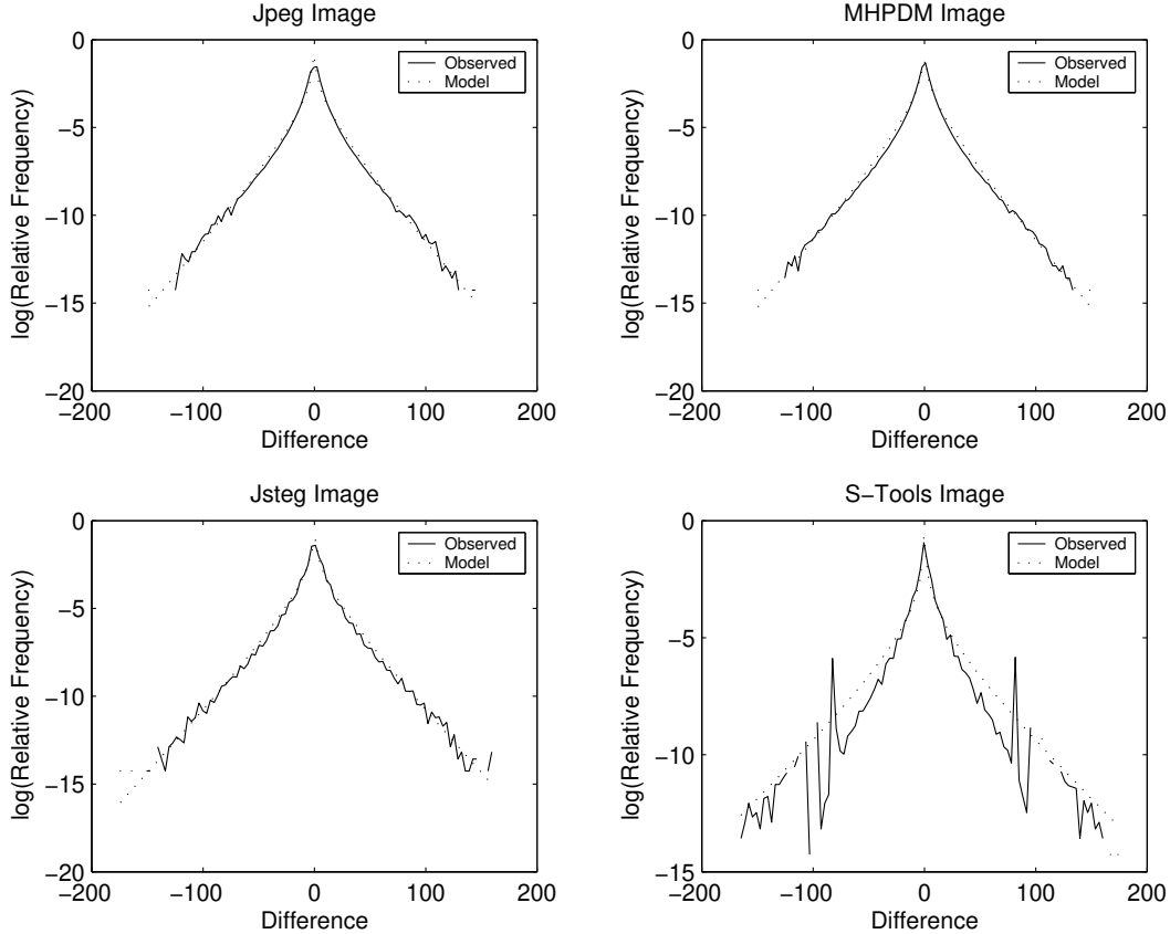
Figure 3: PC Model fit to four versions of the same image. When the message is embedded using the S-Tools algorithm, this can be easily detected due to its discrepancy with the model. For MHPDM and Jsteg stego algorithms, there is a good fit to the natural images model.
