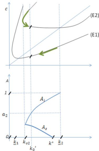
Figure 18. \mu_4 \leq \mu < \mu_0 (pattern V)
