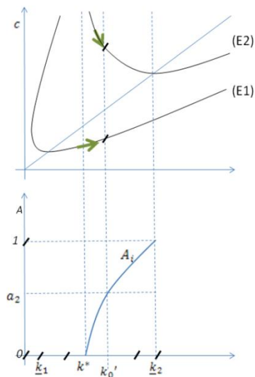
Figure 19. \mu_0 \leq \mu (pattern VI)
