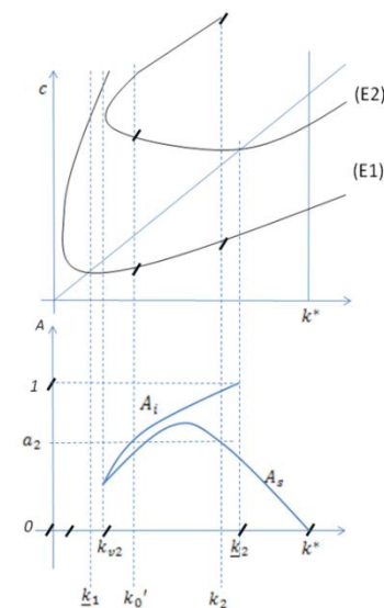
Figure 16. \mu_2 \leq \mu < \mu_3 (pattern III)
