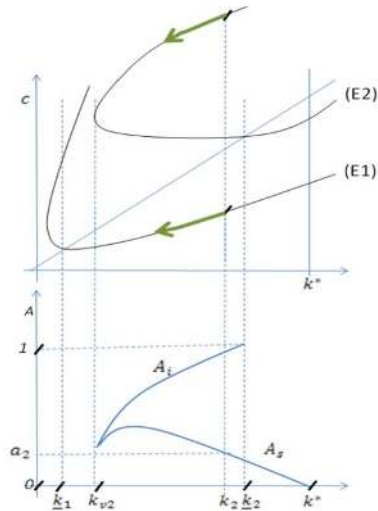
Figure 17. \mu_3 \leq \mu < \mu_4 (pattern IV)
