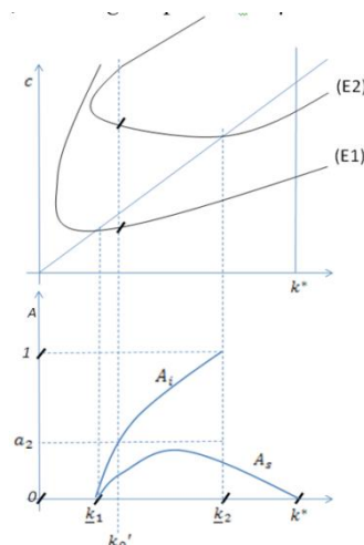
Figure 23: 0 \leq \mu < \mu_3' (pattern II)
