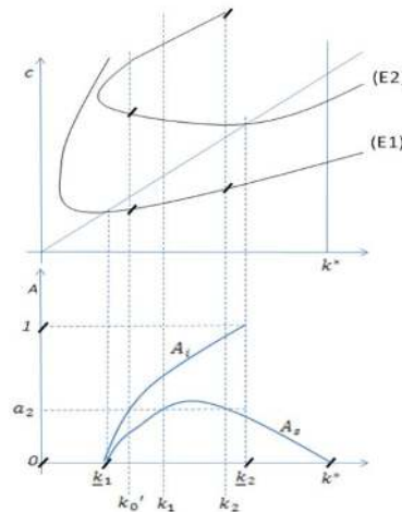
Figure 15. 0 \leq \mu < \mu_2 (pattern I)
