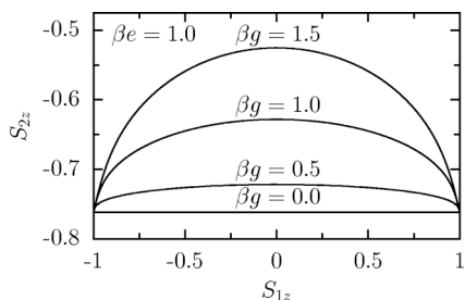
FIG. 2. The Bloch vector component S_{z2} as a function of S_{z1} resulting from Eq. (28) for \beta e=1 and different values \beta g = 0, 0.5, 1, 1.5 . Note that a strictly linear dependence results only for the case of vanishing coupling g=0 . An approximate linear regime exists in a neighborhood of S_{1z}=0 .
