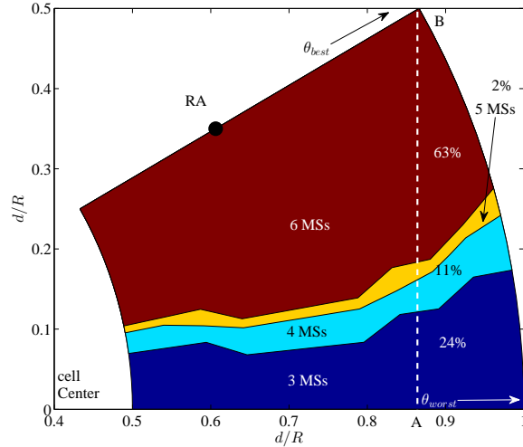
Fig. 12. The number of simultaneously supported MSs satisfying the QoS of SIR > 15 dB.
