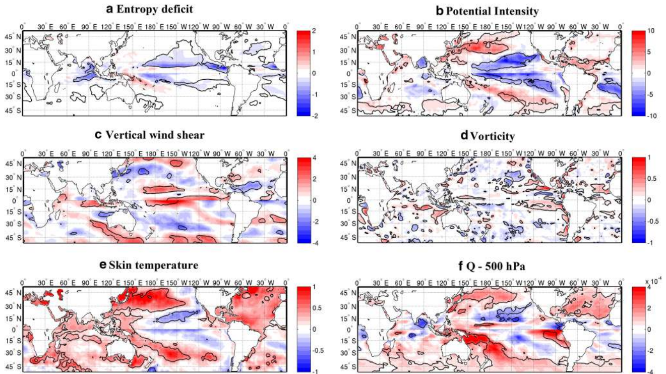
Fig. 1 Seasonal mean differences between 1997 and 2013 and 1980–1996 for: a entropy deficit, b PI, c shear, d vorticity, e skin temperature and f specific humidity at 500 hPa for MERRA reanalysis,
