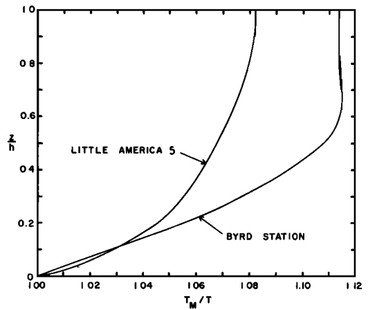
Fig. 5. Reciprocal homologous temperature T_M/T versus normalized ice thickness z/h down the Little America 5 and Byrd Station coreholes. (From Bender and Gow [1961] and Gow et al. [1968].)
