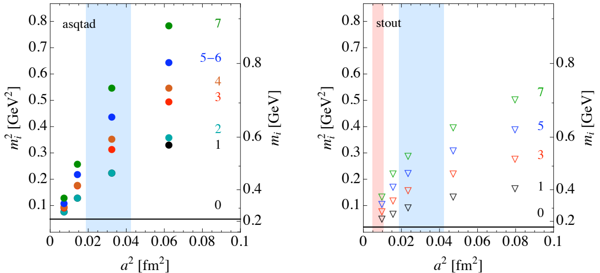
Figure 2: Masses of the pion multiplet squared, as functions of the lattice spacing squared. Left panel: asqtad action [19]. Right panel: stout action. The numbers next to the data correspond to the taste matrices, as listed in Table 1. In both panels, the blue band indicates the relevant range of lattice spacings for a thermodynamics study at N_t = 8 between T = 120 and 180 MeV. The red band in the right panel corresponds to the same temperature range and N_t = 16 . In both figures, the horizontal line labelled as “0” is the pseudo-Goldstone boson, which has a mass of 220 MeV for the asqtad results, and 135 MeV for the stout ones (As we mentioned the splitting is formally proportional to \alpha_s a^2 . At present accuracies and for illustrative purposes the subdominant logarithmic dependence can be omitted).
