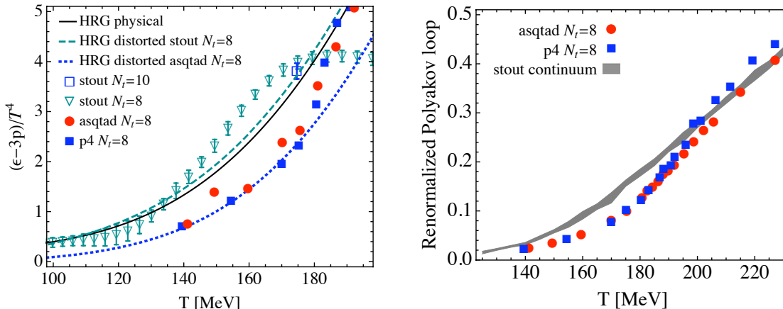
Figure 7: Left: (\epsilon - 3p)/T^4 as a function of the temperature. Open symbols are our results. Full symbols are the results for the asqtad and p4 actions at N_t = 8 [5]. Solid line: HRG model with physical masses. Dashed lines: HRG model with distorted spectrums. As it can be seen, the prediction of the HRG model with a spectrum distortion corresponding to the stout action at N_t = 8 is already quite close to the physical one. The error on the recent preliminary HISQ result [11] is larger than the difference between the stout and asqtad data, that is why we do not show them here. Right: renormalized Polyakov loop. We compare our results with those of the hotQCD Collaboration (asqtad and p4 data for N_t = 8 [5]).
