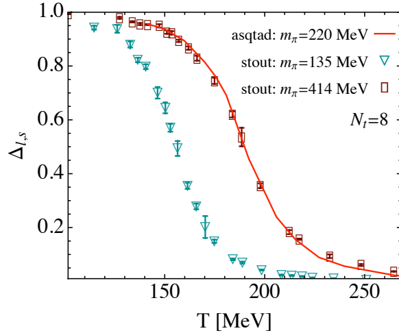
Figure 8: Left: Renormalized chiral condensate as defined in Eq. (4.3). Right: Subtracted chiral condensate \Delta_{l,s} as defined in eq. (4.4), as a function of the temperature. Gray bands are the continuum results of our collaboration, obtained with the stout action. Full symbols are obtained with the asqtad and p4 actions [5, 11]. In both panels, the solid line is the HRG model result with physical masses. The error band corresponds to the uncertainty in the quark mass-dependence of hadron masses. The dashed lines are the HRG+ \chi PT model result with distorted masses, which take into account the discretization effects and heavier quark masses used in [5, 11] for N_t = 8 and N_t = 12 .
