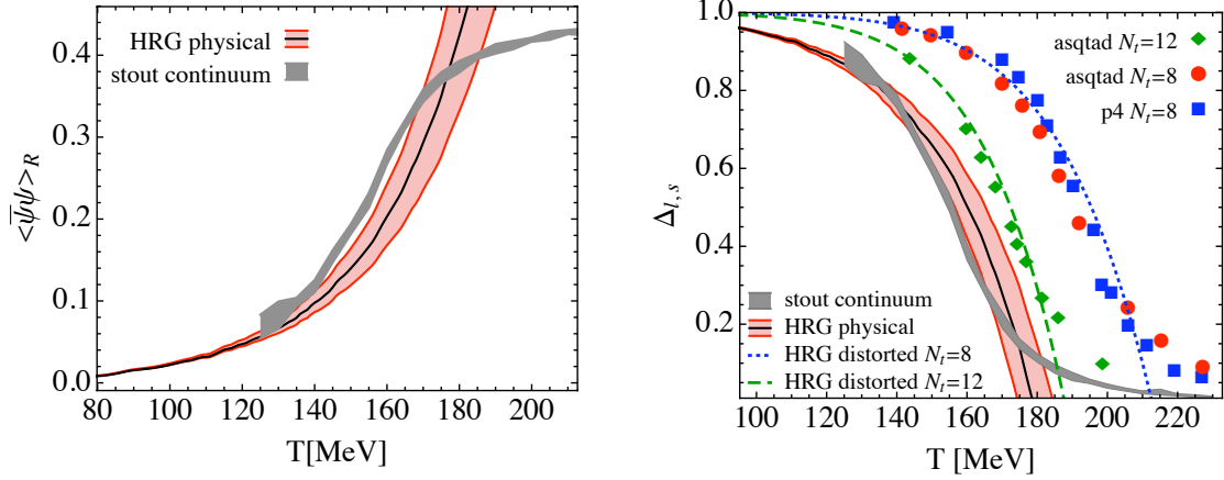
Figure 8: Left: Renormalized chiral condensate as defined in Eq. (4.3). Right: Subtracted chiral condensate \Delta_{l,s} as defined in eq. (4.4), as a function of the temperature. Gray bands are the continuum results of our collaboration, obtained with the stout action. Full symbols are obtained with the asqtad and p4 actions [5, 11]. In both panels, the solid line is the HRG model result with physical masses. The error band corresponds to the uncertainty in the quark mass-dependence of hadron masses. The dashed lines are the HRG+ \chi PT model result with distorted masses, which take into account the discretization effects and heavier quark masses used in [5, 11] for N_t = 8 and N_t = 12 .
