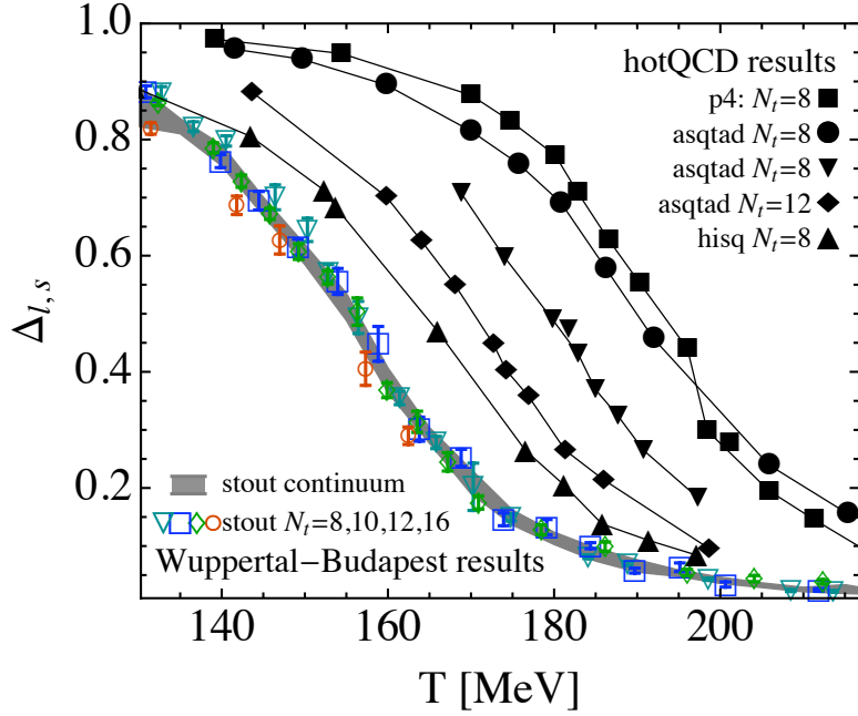
Figure 10: The subtracted chiral condensate \Delta_{I,s} as a function of the temperature. We show a comparison between stout, asqtad, p4 and HISQ [5, 11] results. Our results are shown by colored open symbols, whereas the hotQCD results are shown by full black symbols. The gray band is our continuum result, the thin lines for the hotQCD data are intended to lead the eye. Our stout results were all obtained by the physical pion mass of 135 MeV. The full dots and squares correspond to m_\pi = 220 MeV, the full triangles and diamonds correspond to m_\pi = 160 MeV of the hotQCD collaboration.
