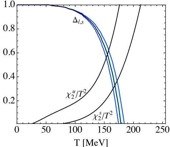
Figure 5: HRG + \chi PT results for the light and strange quark number susceptibilities and the subtracted chiral condensate \Delta_{l,s} . For this last quantity, the error band indicates the uncertainty on the quark mass-dependence of hadrons, see the Appendix. The results have been obtained with physical values for the hadron and resonance masses, thus no lattice artefact has been included.
