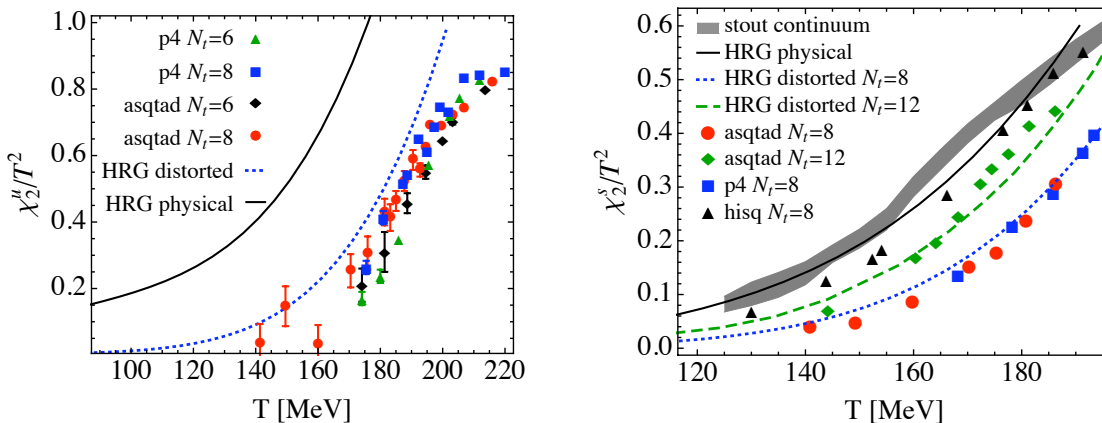
Figure 6: Left: light quark susceptibility as a function of the temperature. Right: strange quark susceptibility as a function of the temperature. In both panels, the points with different symbols correspond to results obtained with the asqtad and p4 actions [5, 11]. The solid line is the HRG model result with physical masses. The dashed and dotted lines are the HRG model results with distorted masses corresponding to N_t = 12 and N_t = 8 , which take into account the discretization effects and heavier quark masses, which characterizes the results of the hotQCD Collaboration. Our continuum result for the strange susceptibility is shown by the band. Good agreement is found with the physical HRG+ \chi PT results. (Due to the noisy contribution of the disconnected diagrams we have not determined the light quark susceptibility.)
