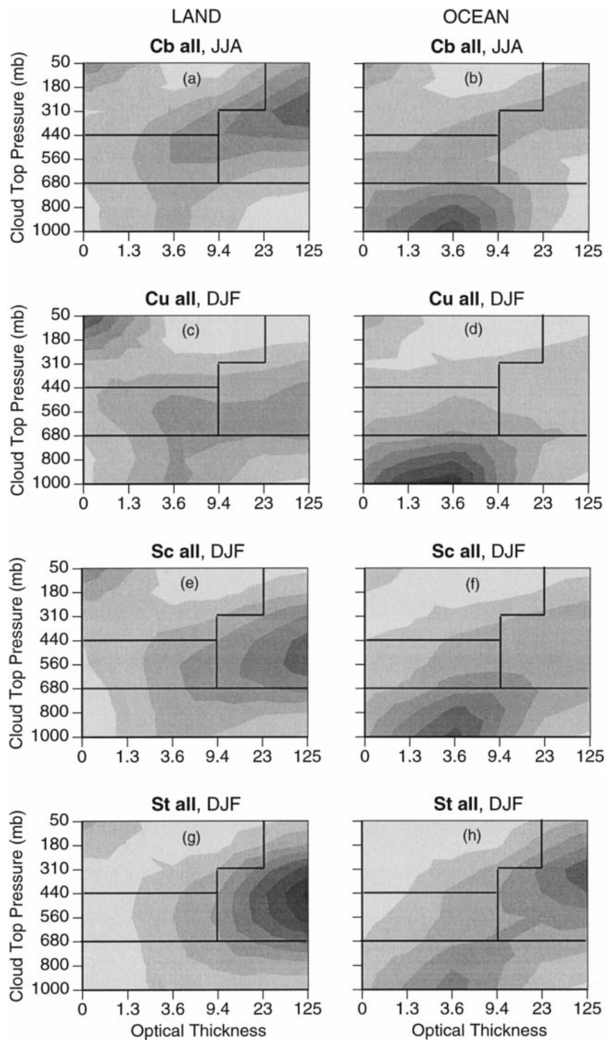
FIG. 8. Distributions of (\tau, p_c) for surface reports of low clouds, irrespective of whether other clouds are also present (the “all” cases), for DJF in the zone 30^\circ\text{--}45^\circ\text{N} , except that JJA statistics are shown for Cb because Cb is more common in summer. The grayscale is defined in Fig. 6.
