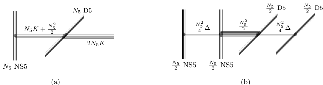
Figure 4. Brane configurations for representative non-gravitating bath solutions (left) and gravitating bath solutions (right). Hanany-Witten transitions can be used to make the 3d quiver gauge theories more apparent, as in figures 2, 3. The numbers of D3-branes on the right are controlled by \delta through \Delta = \frac{1}{2} + \frac{2}{\pi} \arctan e^{2\delta} .
