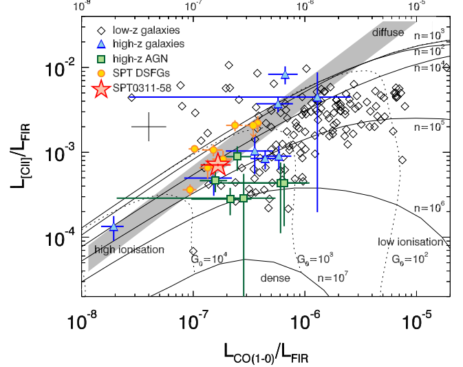
Figure 3. L_{[\text{C II}]} / L_{\text{FIR}} vs. L_{\text{CO}(1-0)} / L_{\text{FIR}} with PDR models adapted from Gullberg et al. (2015). The red star shows how SPT0311–58 falls within the larger SPT DSFG sample. The typical error bar for the low-redshift sample is presented by the black cross.
