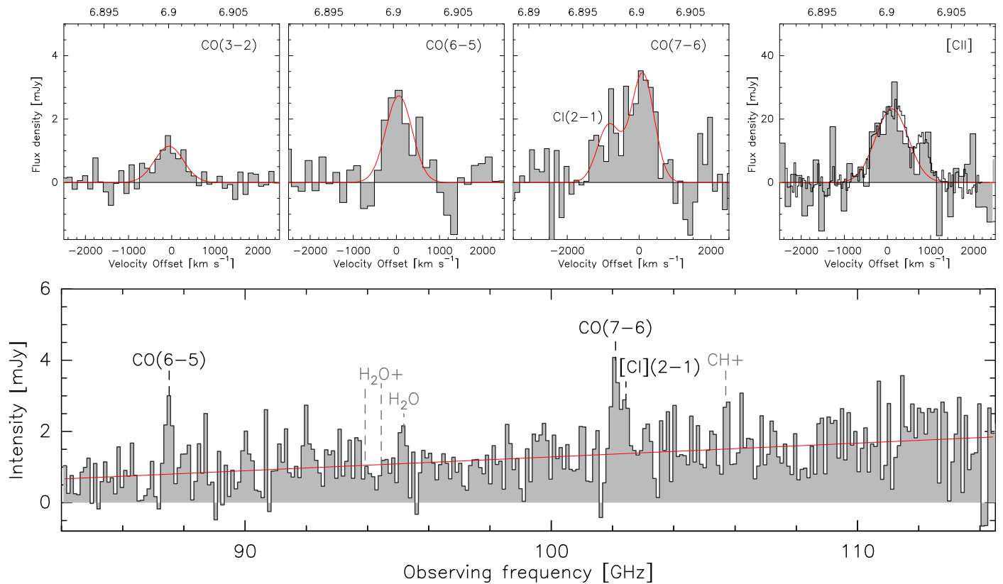
Figure 1. The lower part of the figure shows the ALMA 3 mm spectrum of SPT0311–58 spanning 84.2–114.9 GHz. The spectrum has been binned to best show the lines. Transitions labeled in black are detected, and gray labels indicate where other transitions should be. The red line indicates the zeroth-order baseline. The sub-panels above the spectrum show, from left to right, the continuum-subtracted spectra of ATCA CO(3–2), ALMA CO(6–5), ALMA CO(7–6) and C I(2–1), and APEX [C II] with ALMA [C II] overlaid as a solid black histogram. Gaussian fits to the spectra are shown in red.
