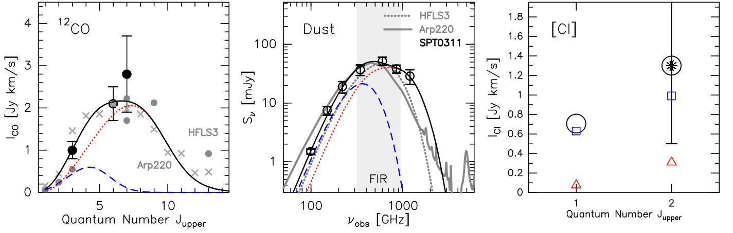
Figure 2. Results of simultaneous fitting of the CO-SLED (left), SED (middle), and [C I] (right) line flux. The CO line intensities are plotted as filled circles, the continuum fluxes as open circles and the [C I] flux as an asterisk. The blue dashed line and squares show the cold component, the red dotted line and triangles show the warm component, the black solid line and circles (in the right panel) show the combination of the two components. In gray is shown similar data for HFLS3 (dots and dotted line) and Arp220 (crosses and solid line), normalized to the CO(6–5) flux of SPT0311-58 for the CO-SLED and to the peak of the continuum SED of SPT0311-58 for the SED. The line fluxes and continuum properties fitted are listed in Table 2. Left: two-component CO-SLED. Middle: two-component SED fitting based. Right: the contribution of each of the two components to the [C I](2–1) line and predictions for the [C I](1–0) line.
