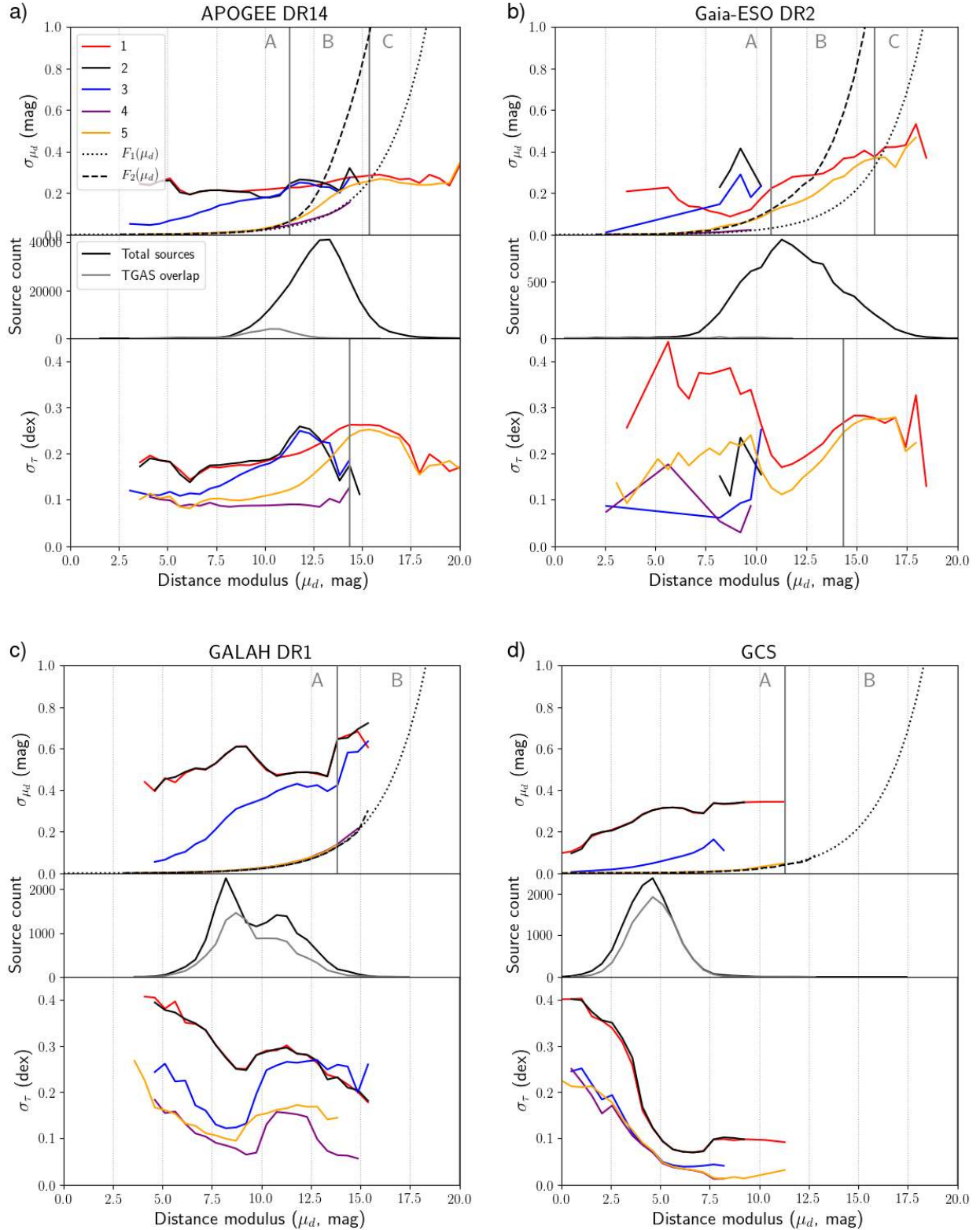
Fig. C.1. As in Fig. 1. We note that for SEGUE survey (subplot j), there are no stars with TGAS parallaxes.
