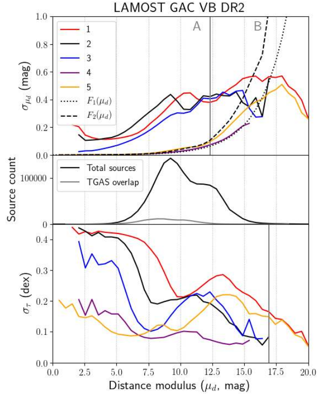
Fig. 1. Distance modulus uncertainties \sigma_{\mu_d} (top panel) and log(age) uncertainties \sigma_{\tau} (bottom panel) as functions of the distance modulus. Lines show median values in 0^m.5 distance modulus bins. Colours are for datasets: dataset 1 – complete survey (red); dataset 2 – TGAS overlap (black); dataset 3 – TGAS overlap with TGAS parallaxes (blue); dataset 4 – TGAS parallaxes with EoM precisions (magenta); dataset 5 – UniDAM parallax with EoM precisions (orange). We show only distance modulus bins with at least five stars so as to reduce the noise. Therefore, the distance modulus range presented can differ for different datasets, especially for surveys with small overlap with TGAS. The dotted black line shows F_1(\mu_d) , the dashed black line shows F_2(\mu_d) (as described in Sect. 4.1). Vertical grey lines and grey labels at the top panel mark borders between ranges A, B, and C (see Sect. 4.1 for details). Vertical grey line at the bottom plot marks maximum distance modulus for which the use of parallaxes gives at least 10% improvement in log(age) uncertainty (see Sect. 4.2). Middle panel: total number of stars in the survey (black) and the number of stars in overlap with TGAS (grey) as a function of distance modulus.
