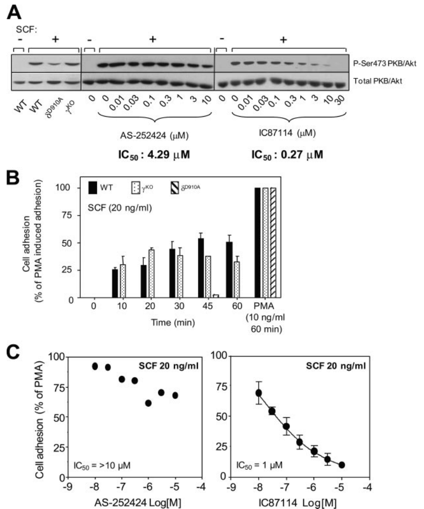
FIGURE 3. Effect of p110 \gamma or p110 \delta inhibition on SCF-dependent Akt/PKB phosphorylation and adhesion of mast cells. A , (Left panel) \gamma^{KO} and \delta^{D910A} BMMCs were stimulated with SCF or vehicle (control) and Akt/PKB phosphorylation assessed by western blotting as described in Materials and Methods . A representative blot of two independent experiments is shown. (Middle and right panels), BMMCs were pretreated for 30 min with varying concentrations of inhibitors, followed by stimulation with SCF for 5 min and immunoblotted for Akt/PKB (phospho-Ser473 or total). IC 50 values were determined by ratiometric analysis of immunoblots (data not shown), as described in the legend to Fig. 2. A representative immunoblot of three independent experiments is shown. B , Impact of genetic inactivation of PI3K isoforms on SCF-dependent mast cell adhesion. The experiment shown is representative of five independent experiments. C , Impact of pharmacologic inactivation of PI3K isoforms on SCF-dependent mast cell adhesion. Graphs show data from a representative experiment done at least three (AS-2252424) or two (IC87114) times, with identical results.
