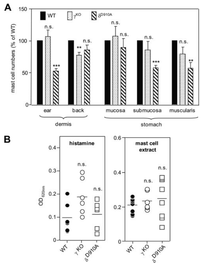
FIGURE 1. Impact of genetic inactivation of p110 \gamma or p110 \delta on mast cell numbers and vascular permeability responses in vivo . A , Mast numbers in different anatomical locations. Depending on the anatomical location, the units for counting were as follows: ear dermis: per 5 mm length, beginning at the ear tip; stomach: per one complete sagittal section; and back dermis: unit is per 10 high power fields ( \times 40 objective = \times 400 magnification). Exclusively, dermal mast cells (those found among dermal collagen) were counted for each mouse; s.c. mast cells (those found among fat cells of the subcutis) were not counted, as thickness of the s.c. fat can vary greatly among animals depending on body condition. Data are presented as mast cell numbers expressed as % of WT ( n = 5 for all genotypes). The mast cell distribution in \delta^{D910A} mice has been published previously (17) and is presented here for comparative purposes. B , Effect of vasoactive stimuli on vascular leakage in PI3K mutant mice. Numbers of mice used were as follows: histamine: WT, \gamma^{KO} , and \delta^{D910A} , n = 6 each; and mast cell extract: WT, n = 8 ; \gamma^{KO} , n = 6 ; and \delta^{D910A} , n = 8 .
