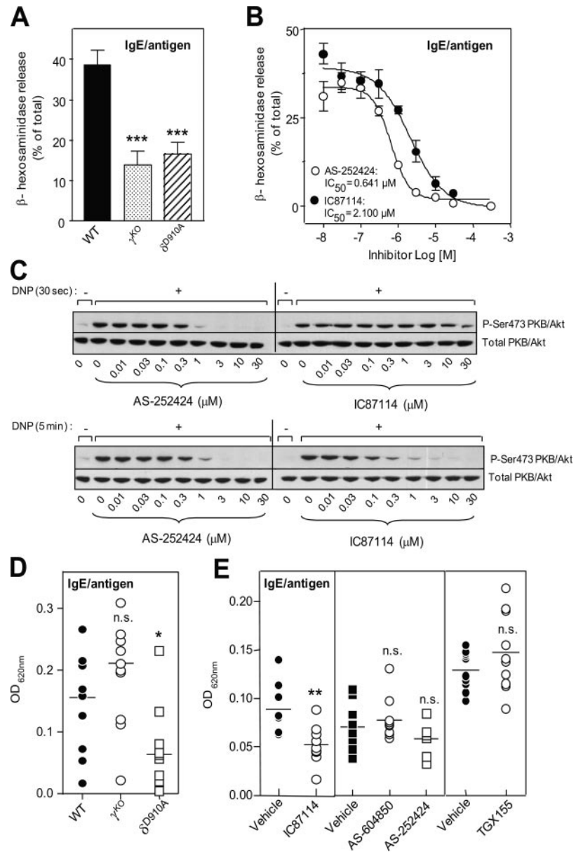
FIGURE 4. Effect of p110 \gamma or p110 \delta inhibition on IgE-dependent in vitro mast cell degranulation, Akt/PKB phosphorylation, and PCA response in vivo . A , Effect of genetic inactivation of p110 \gamma or p110 \delta on IgE/Ag-induced BMMC degranulation in vitro . Graph shows the mean \pm SD of the following number of independent experiments: WT, n = 10 ; \delta^{D910A} , n = 10 ; and \gamma^{KO} , n = 8 ; done in quadruplicates. Mean \pm SD spontaneous hexosaminidase release for experiments was as follows: WT, 8.23\% \pm 1.83 ( n = 10 ); \delta^{D910A} , 11.88\% \pm 1.9 ( n = 10 ); and \gamma^{KO} , 8.0\% \pm 1.4 ( n = 8 ). B , Effect of isoform-selective PI3K inhibitors on IgE/Ag-induced BMMC degranulation in vitro . Graph shows data from two independent experiments \pm SEM. C , Impact of PI3K inhibitors on IgE/Ag-induced Akt/PKB phosphorylation upon 30-s ( top panel ) and 5-min ( bottom panel ) stimulation of IgE-sensitized mast cells with Ag. A representative blot from three independent experiments is shown. D , PCA response of WT and gene-targeted mice (WT, \gamma^{KO} , and \delta^{D910A} ; n = 11 each). E , PCA responses of WT mice treated with PI3K inhibitors. Numbers of mice used were as follows: left panel : IC87114 (p110 \delta inhibitor): vehicle, n = 8 and IC87114, n = 9 ; middle panel : AS-604850 and AS-252424 (p110 \gamma inhibitors): vehicle, n = 9 , AS-604850, n = 10 , and AS-252424, n = 8 ; and right panel : TGX-155 (p110 \beta inhibitor): vehicle, n = 10 and TGX-155, n = 10 .
