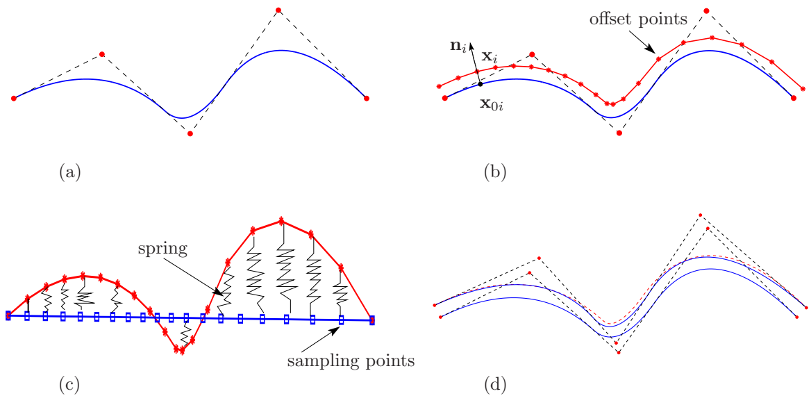
Figure 1: The proposed algorithm to create an offset curve of a given B-spline curve: (a) the original curve, (b) a set of offset points is generated, (c) sampling points on the initial guess offset curve and a system of springs connecting those sampling points and the offset points and (d) the final offset curve is obtained when the energy of the spring is minimum.
