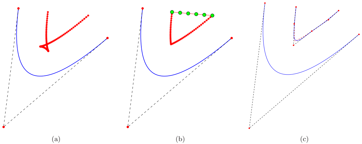
Figure 5: A cubic Bézier curve with radius of curvature less than the offset distance : (a) offset points with local intersection (b) after removing and (c) offset curve.
