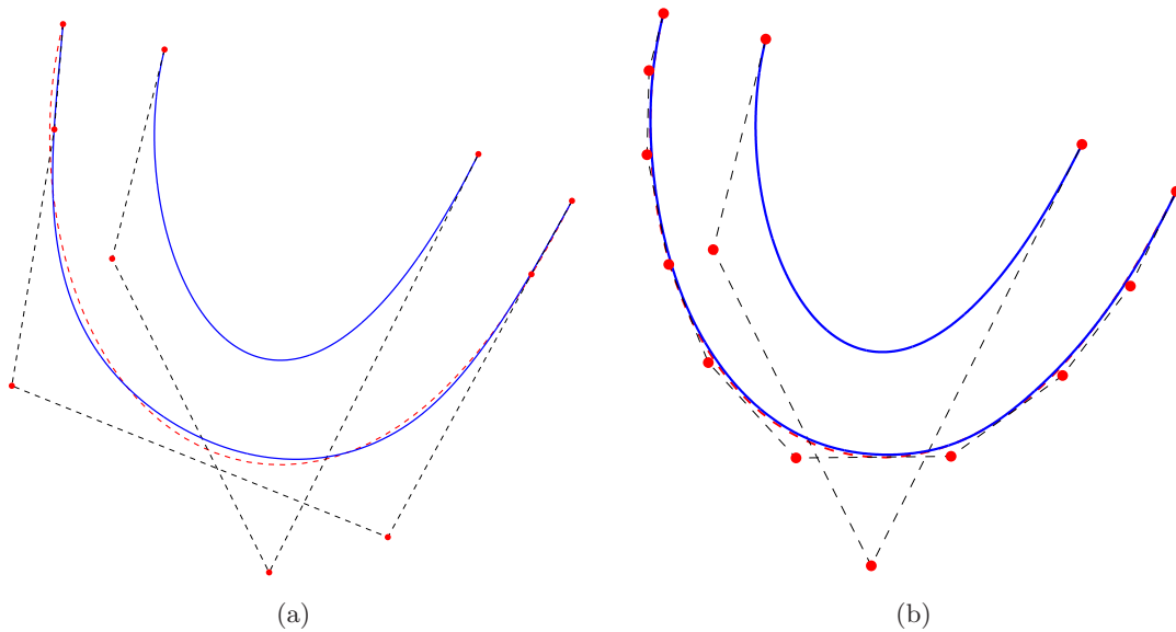
Figure 3: Cubic Bézier curve example: (a) offset curve has the same number of CPs as the original curve and (b) offset curve has 10 CPs. The dotted lines denote the "exact" offset curve that joins the offset points.
