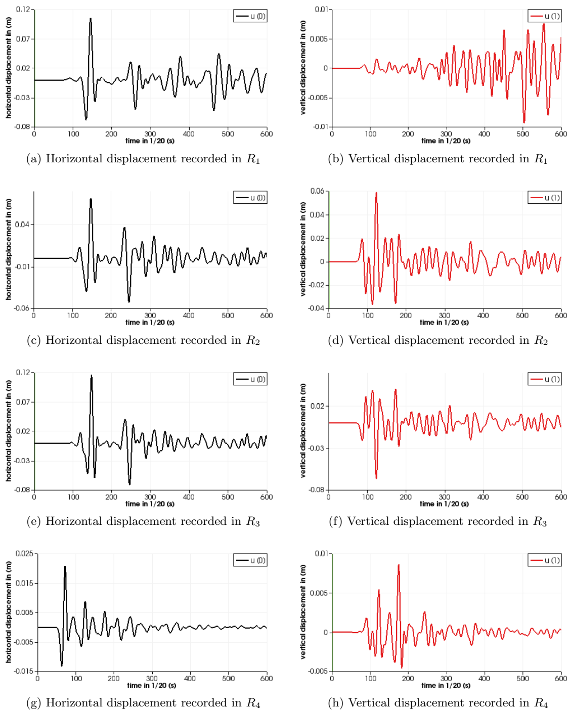
Figure 16: Computed horizontal u_1 and vertical u_2 displacements ( [m] ) vs. time t (scaled as 1/20 s ) at the four receivers stations R_1 , R_2 , R_3 , and R_4 highlighted in Fig. 14 (the displacements magnitudes are on different scales).
