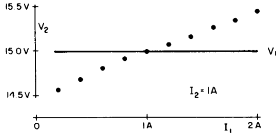
Fig. 11 Cross-regulation property of the circuit of Fig. 10: variation of V_2 as a function of I_1 , with V_1 and I_2 maintained constant.
