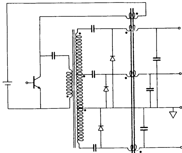
Fig. 9 Any or all of the input and output inductors in the multiple-output new converter can be coupled, which permits the switching current ripple to be "steered" towards or away from a given terminal.
