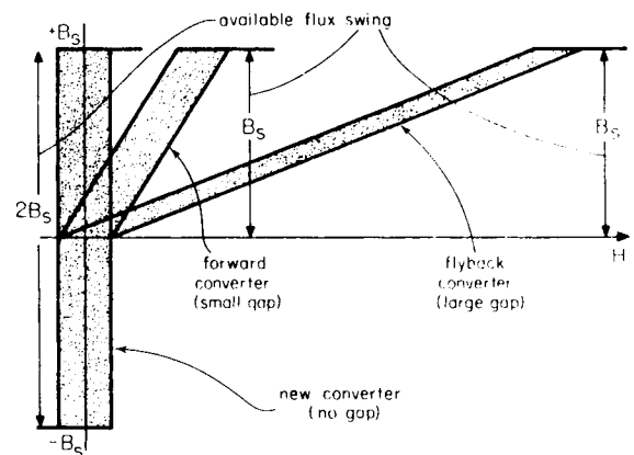
Fig. 7 Comparison of isolation transformer core utilization in the new converter and the forward and flyback converters. Twice the flux swing is available in the new converter.
