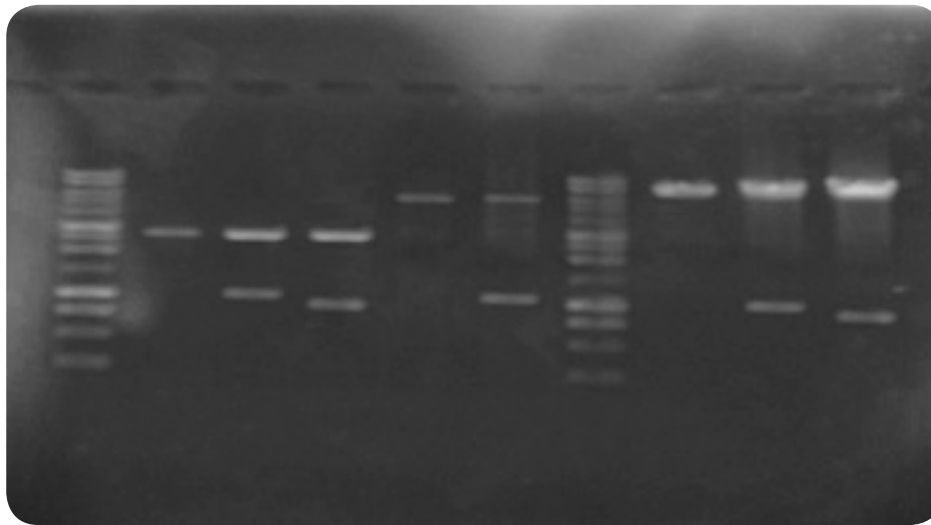
Figure 3. Agarose gel (0.8%) of ribC and parN clones. M: 1kb DNA ladder (Promega); Lane 1: pUCPU21 ( NdeI/BamHI ); lane 2: pUCRC ( NdeI/BamHI ); lane 3: pUCPN ( NdeI/BamHI ); lane 4: pET16b ( NdeI/BamHI ); lane 5: pETRC ( NdeI/BamHI ); lane 6: pUWL201PW ( NdeI/BamHI ); lane 7: pUWRC ( NdeI/BamHI ), lane 8: pUWPN ( NdeI/BamHI )
