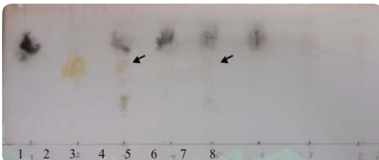
Figure 6. TLC analysis of RibC protein catalyzed conversion of G-6-P into 2-deoxy-scylo-inosose. Lane 1: standard Glucose-6-phosphate; lane 2: standard 2-deoxy-scylo-inosose; lane 3: pETRC 4 hr; lane4: pET16b 4hr; lane5: pETRC 12 hr; lane 6: pET16b 12hr; lane 7: PETRC 4hr, No G-6-P; lane 8: pET16b 4hr, No G-6-P.
