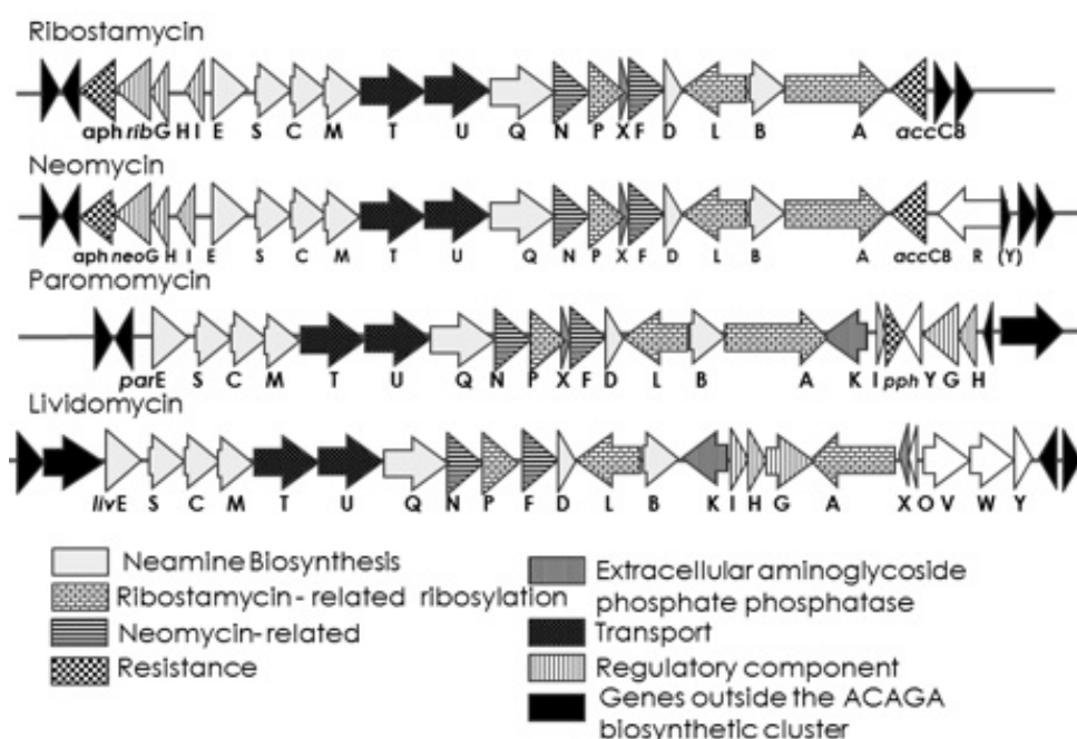
Figure 1. The Biosynthetic gene clusters of the Neo family of ACAGAs.[1.: Ribostamycin biosynthetic gene cluster (Accession code = AJ744850.1); neomycin biosynthetic gene cluster (Accession code = AJ629247.1); paromomycin biosynthetic gene cluster (Accession code = AJ628955.2); lividomycin biosynthetic gene cluster (Accession code = AJ748832.1).
