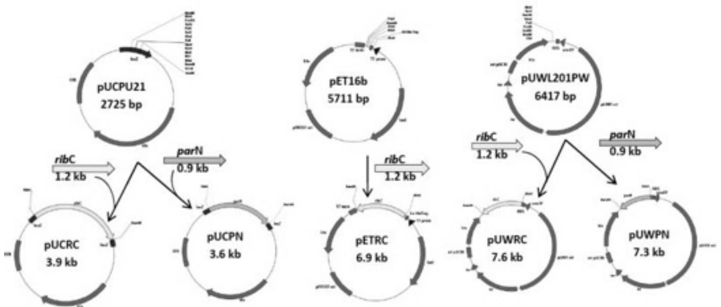
Figure 4. Schematic diagram of ribC and parN clones generated in this study.
