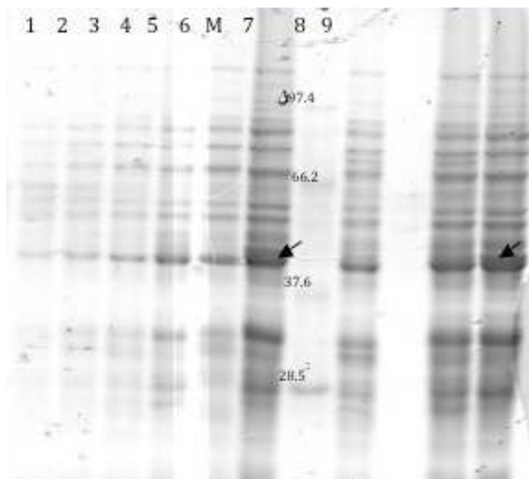
Figure 5. Laemmli SDS-PAGE gels(12%) of the cell-free extracts of E. coli JM109(DE3) harboring the following plasmids: pET16b, lane 1 (before induction), lanes 3, 5, 7, 8 were, 2 hr, 4 hr, 12 hr, 12hr after IPTG induction; pETRC (RibC), lane 2 (before induction), lanes 4, 6, 9 were 2 hr, 4 hr, 12hr after IPTG induction. M: protein marker in kDa (Jena Bioscience). Arrows point to the protein bands corresponding to the expected molecular mass of the RibC protein.
