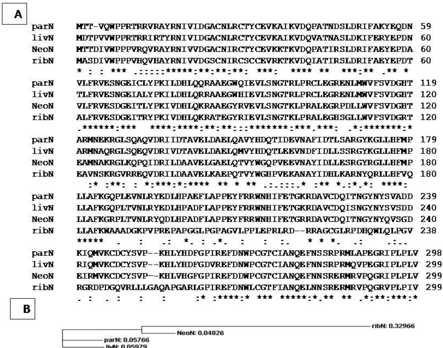
Figure 2. (A) Alignment of RibN and its homologous proteins (accession code = CAG34032) and the homologous proteins: ParN (accession code = CAF32379), livN (accession code = CAG38702) and NeoN (accession code = CAF33317) and (B) their phylogram.
