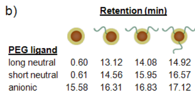
Figure 4. (a) AE-HPLC retention of free DNA compared with DNA conjugated to 5 nm AuNP. At all DNA lengths, free DNA is retained more strongly than 5 nm AuNP conjugated to one or two strands of the same DNA. Peak width at half the maximum value is approximately 4 mM for DNA and 20 mM for mono- and di-conjugate. (b) Ligand used to passivate gold surface plays an important role in conjugate retention, although in each case, increasing numbers of DNA strands correlate with increased retention.
