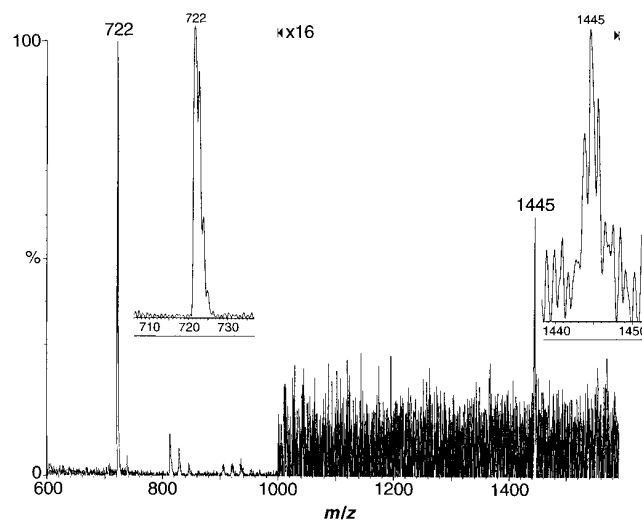
Fig. 1. Electrospray MS (+) spectrum of a 0.02 to 0.05 mM solution of (\text{C}_{59}\text{N})_2 in toluene. The insets are expansions around the 722 and 1445 m/z peaks. The expanded patterns give an excellent fit to the calculated isotope mass ratios.
