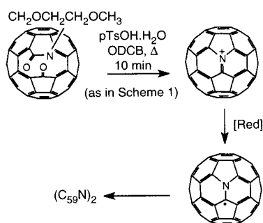
Scheme 2. Proposed cascade of events in the pTsOH.H 2 O-initiated formation of (C 59 N) 2 from N-MEM ketolactam 1 in refluxing ODCB.
