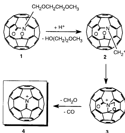
Scheme 1. Proposed mechanism for the gas-phase formation of azafullerone ion C_{59}N^+ (4) from N-MEM ketolactam 1 in FABMS.
