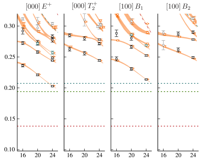
FIG. 11. Spectra ( a_1 E_{\text{cm}} versus L/a_s ) in irreps with \ell = 2 as lowest subduced partial wave, as described by the amplitude given in Eq. (4). Black/blue points show the lattice QCD spectrum of Fig. 3 and orange curves and points (displaced slightly for clarity) the result of the fitted amplitude. Long dashed lines indicate the position of noninteracting meson-meson levels corresponding to operators that were not included in the variational basis.
