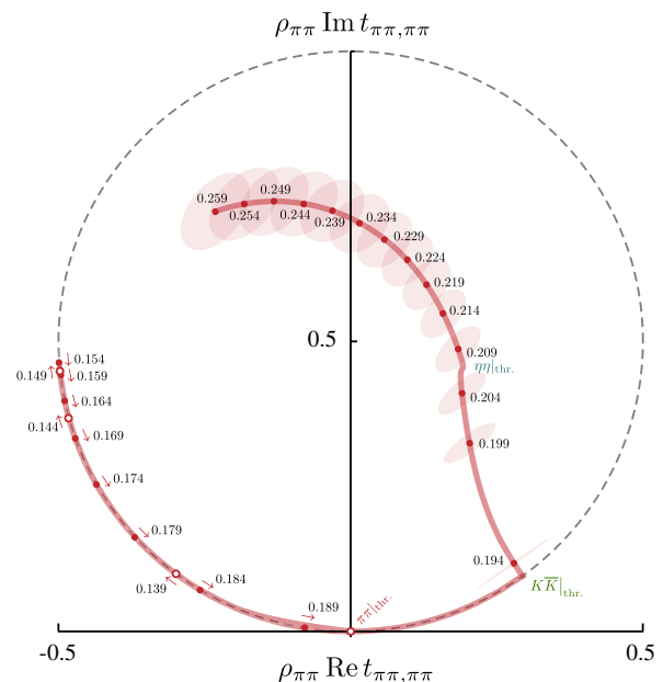
FIG. 9. Argand diagram representation of the t_{\pi\pi,\pi\pi} element of the amplitude given by Eq. (3). Points are spaced evenly in energy with a_t \Delta E_{cm} = 0.005 . The amplitude initially moves clockwise from \pi\pi threshold (open circles) before doubling back upon itself (closed circles).
