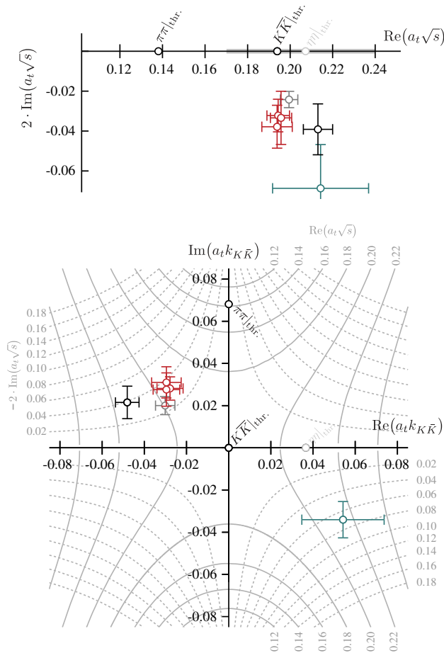
FIG. 19. Poles of two-channel ( \pi\pi , K\bar{K} ) amplitudes described in the text describing energy levels in the region 0.17 < a_t E_{\text{cm}} < 0.24 excluding “ \eta\eta ” levels. Black point shows the pole of the three-channel amplitude described by Eq. (3). Gray point shows the pole from a typical amplitude taken from Sec. IV A 3 where three-channel amplitudes described all levels in the region 0.17 < a_t E_{\text{cm}} < 0.24 . Remaining colored points correspond to the amplitudes described in the text and plotted in Fig. 18.
