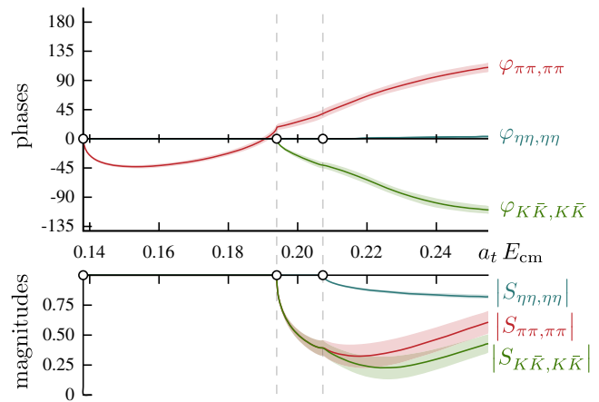
FIG. 8. Phases and magnitudes of diagonal elements of the S -matrix, S_{ii}(E_{cm}) = |S_{ii}(E_{cm})| e^{2i\varphi_{ii}(E_{cm})} , for the amplitude given by Eq. (3).
