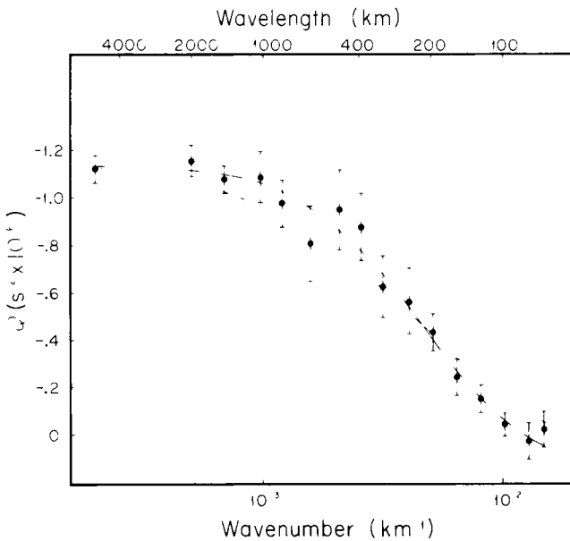
Figure 1. Isostatic response estimates for the United States. Bars represent ±1 standard error in the data. Continuous curve is the response of the local compensation model with both negative and positive densities; dashed curve is the response of the local compensation model with only negative densities and smallest one-norm misfit to the data.
