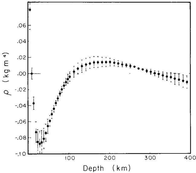
Figure 2. Isostatic density model for the USA, obtained by inverting the response data in Fig. 1, assuming local compensation. Ordinate is density contrast per unit topographic elevation.
