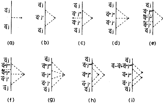
FIG. 4. Diagrammatic representations of the irreducible phonon self-energy up to fourth order in phonon-isotope scattering. Solid lines represent phonons and dashed lines denote the interactions with the marked isotopes. External phonon lines which are attached for convenience to specify the momentum and polarization should be amputated.
