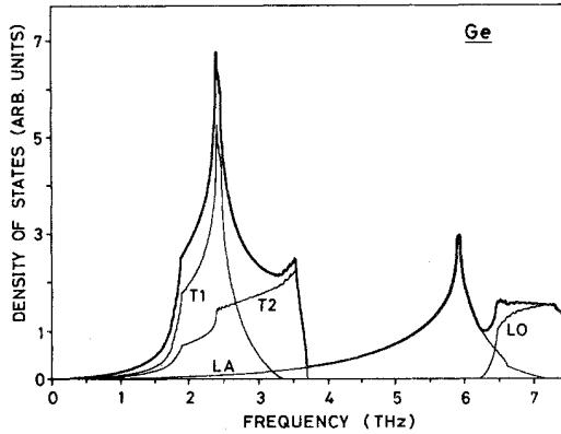
FIG. 2. Computer plot of the phonon densities of states in Ge as a function of frequency up to 7.5 THz. The dynamical matrix has been diagonalized at points \vec{q} , which form a uniform shifted mesh over the \frac{1}{48} irreducible section of the first Brillouin zone. The number of intervals into which we divide the longest q_x axis of the irreducible section is 30. Frequency range is divided into intervals d\nu of width of 1 \times 10^{-3} THz.
