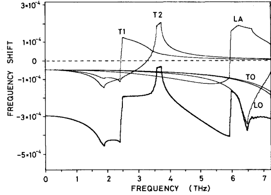
FIG. 5. Computer plot of the frequency shift \Delta\omega/\omega up to 7.25 THz. Each contribution of six branches to \Delta\omega/\omega is also displayed by fine curve. This plot is obtained by dividing the irreducible section of the first Brillouin zone into meshes by the same manner as in obtaining the phonon density of states (Fig. 2), but by dividing the frequency range into intervals d\nu of width 0.01 THz.
