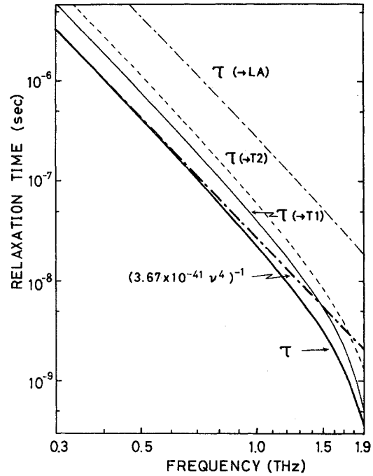
FIG. 3. Frequency dependence of the relaxation time \tau up to 1.9 THz. Contributions to \tau of the scatterings into three acoustic branches are shown with fine curves. Bold dotted-dashed line indicates the \nu^{-4} dependence extrapolated from the low-frequency limit.
