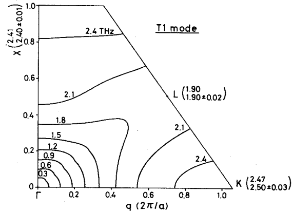
FIG. 1. Calculated constant-frequency curves of the lowest TA phonons, i.e., T1 mode, in the first quadrant of the (1\bar{1}0) plane of Ge. (Frequencies indicated are in units of THz.) Frequencies at zone-boundary points X , L , and K are shown in parentheses, calculated value in the upper row and experimental value in the lower row.
