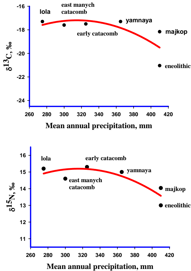
Figure 4 Average values of \delta^{13}\text{C} (above) and \delta^{15}\text{N} (below) for humans as well as annual precipitation.
