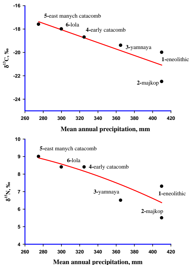
Figure 3 Average values of \delta^{13}\text{C} (above) and \delta^{15}\text{N} (below) for domesticated animals as well as annual precipitation.
