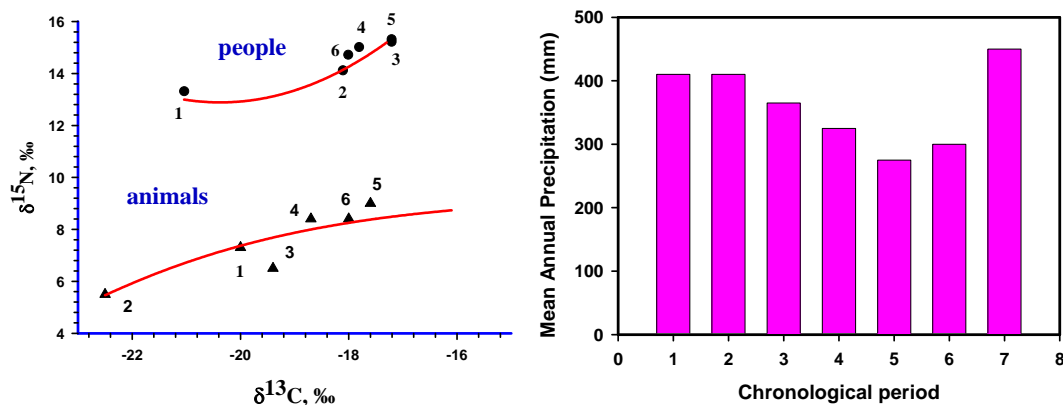
Figure 2 a) Average values of \delta^{13}\text{C} and \delta^{15}\text{N} for human and animal bone collagen from the studied cultures; b) Mean annual precipitation during these archaeological cultures (Demkin et al. 2002). Legend: 1 – Eneolithic; 2 – Majkop; 3 – Yamnaya; 4 – Early Catacomb; 5 – East Manych Catacomb; 6 – Lola and Krivaya Luka; 7 – modern values.
