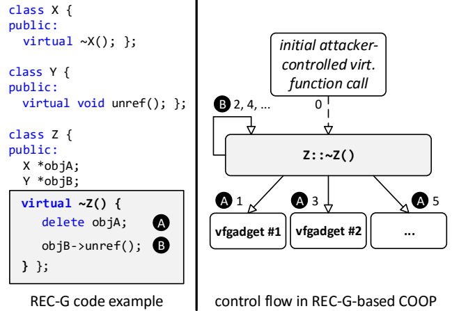
Figure 1: Left: C++ code example of a REC-G ( Z::~~Z() ); right: the corresponding adversary-induced control flow; arrows indicate a calls relationship and are numbered in the order of their execution. The labels A and B refer to the call sites in Z::~~Z() respectively.
