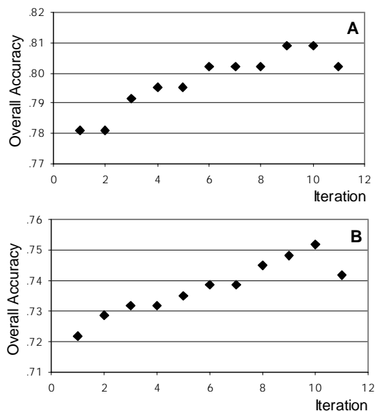
Figure 3: Accuracy results on core objects for each iteration
