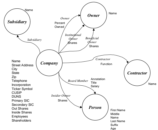
Figure 1: Corporate data ontology
