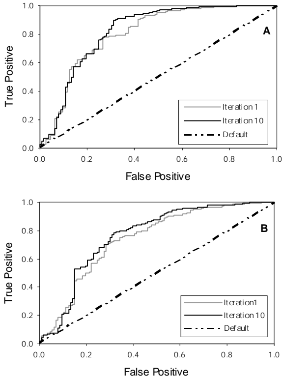
Figure 4: ROC Curves for classification on sample core objects
