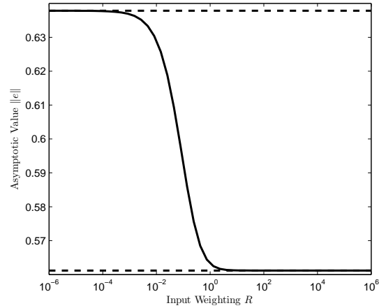
Fig. 10. Effect of different weighting matrices on asymptotic performance
