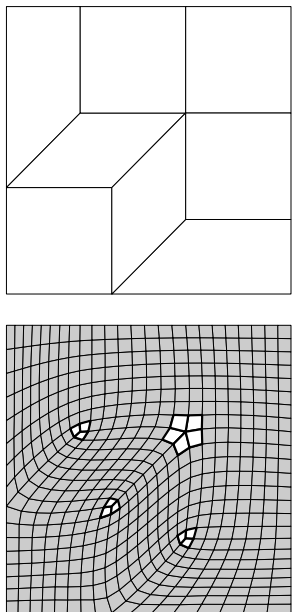
Figure 4: Singularities in the refined net.
