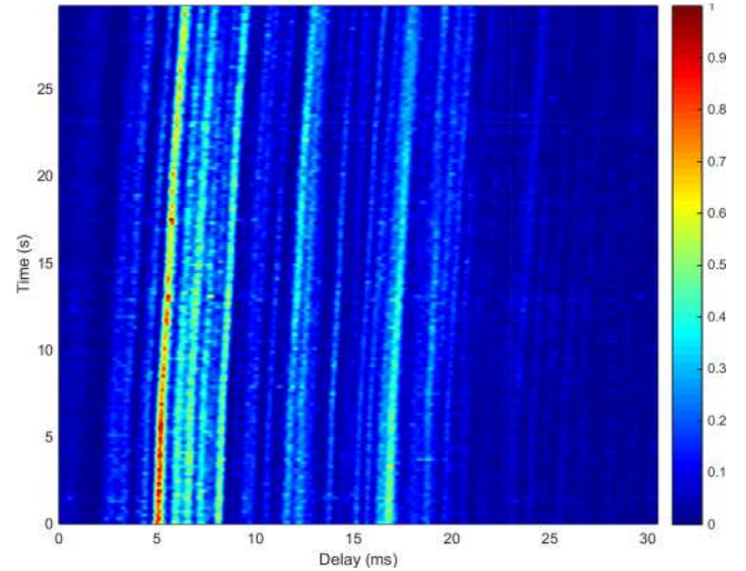
Fig. 11. Time-varying CIR on Channel 01 during 30 s.
