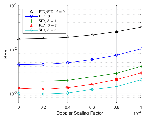
Fig. 9. BER performance comparison between two iterative OSDM detection schemes, i.e., PID and SID.
