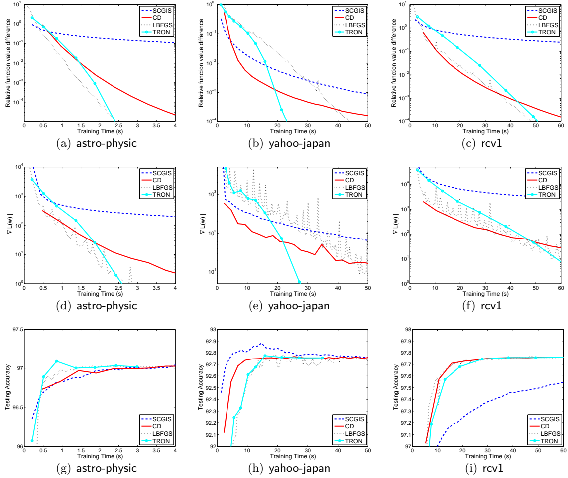
Figure 3: Results on real-valued document data. The first row shows time versus the relative function difference (42). The second and third rows show \|\nabla L(\mathbf{w})\| and testing performances along time, respectively. Time is in seconds.
