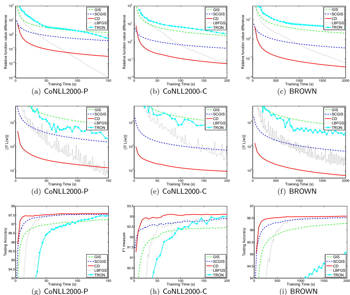
Figure 2: Results on 0/1-featured data. The first row shows time versus the relative function difference (42). The second and third rows show \|\nabla L(\mathbf{w})\| and testing performances along time, respectively. Time is in seconds.
