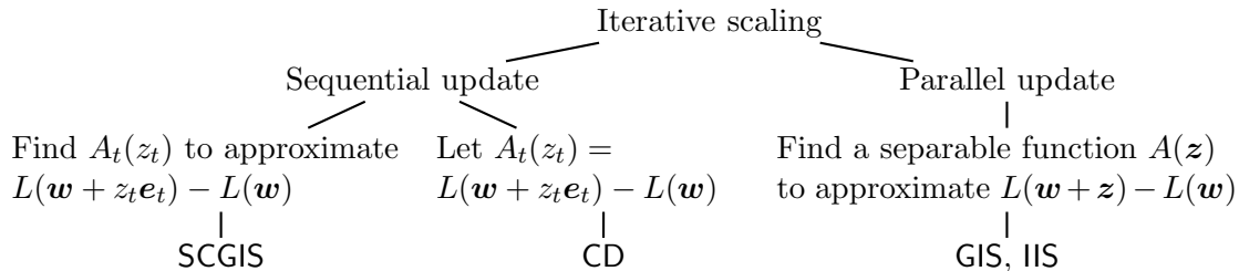
Figure 1: An illustration of various iterative scaling methods.
