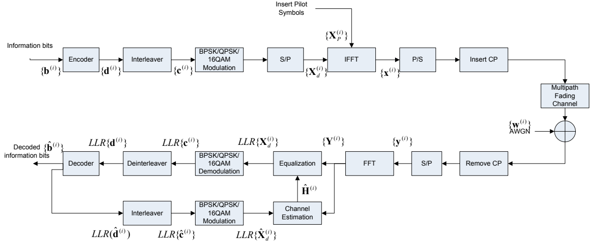
Fig. 2. OFDM system with iterative turbo channel estimation.
