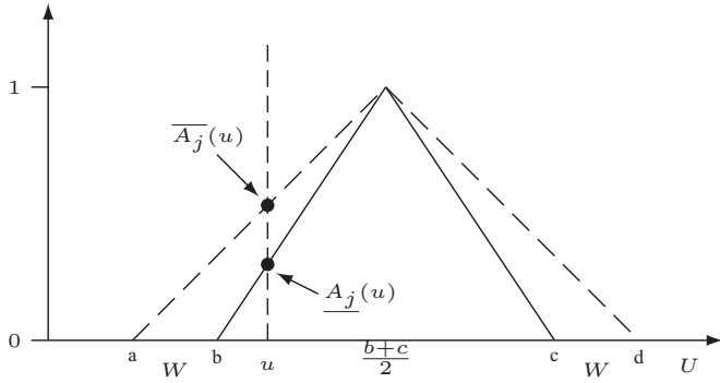
Fig. 3. Example of an initial constructed IVFS as defined in [24] and [34]. The solid line is the initial fuzzy set, and therefore, it is the lower bound of the IVFS. The dashed line is the upper bound of the IVFS.
