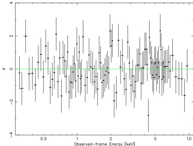
Fig. 4. The broad-band data-to-model residuals (in terms of \sigma ) obtained from the double blackbody phenomenological fit to the EPIC data (see text and Table 1 for details). For clarity, only the highly-binned pn residuals are shown.
