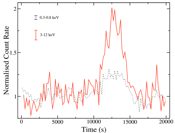
Fig. 7. The 0.3–0.8 keV (black dotted curve) and 3–12 keV (red solid curve) normalised light curves. The vertical lines in the top left of the graph indicate the size of the average error bars. Zero seconds on the time axis marks the start of the observation at 09:18:44 on 2002–06–22.
