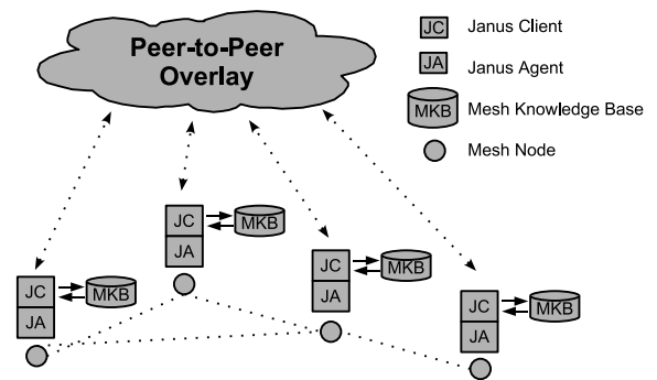
Fig. 2. JANUS Architecture.
