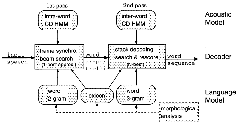
Fig. 2 Block diagram of Japanese dictation system.
