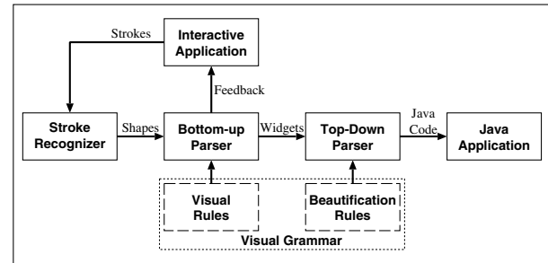
Figure 7: JavaSketchIt architecture
