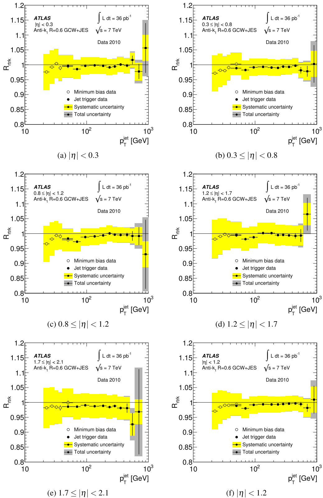
Fig. 59 Double ratio of the track to calorimeter response in data and Monte Carlo simulation, R_{r_{\text{trk}}} = [r_{\text{trk}}]_{\text{Data}}/[r_{\text{trk}}]_{\text{MC}} , for anti- k_r jets with R = 0.6 using the GCW+JES calibration scheme as a function
