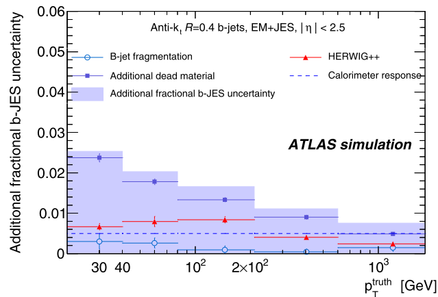
Fig. 86 Additional fractional b -jet JES uncertainty as a function of the truth jet transverse momentum for anti- k_r jets with R = 0.4 calibrated with the EM+JES scheme for |\eta| < 2.5 . Shown are systematic Monte Carlo variations using different modelling of the b -quark fragmentation and physics effects as well as variations in the detector geometry and the uncertainty in the calorimeter response to b -jets as evaluated from single hadron response measurements. Uncertainties on the individual points are statistical only
