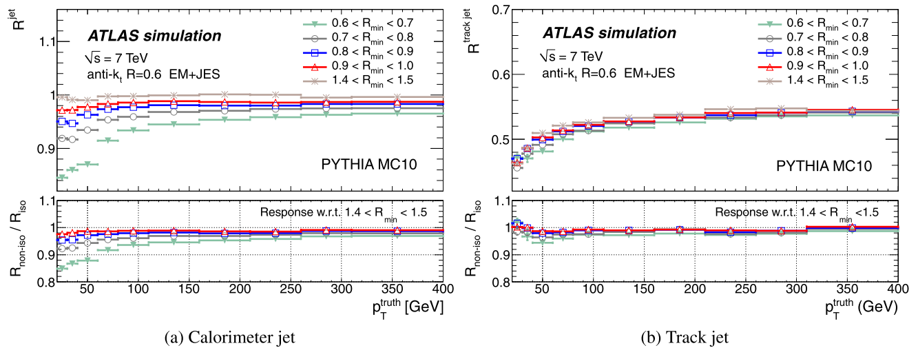
Fig. 73 Average ratio of calorimeter jet (a) and the track jet (b) p_T to the matched truth jet p_T as a function of truth jet p_T for anti- k_t jets with R = 0.6 , for different R_{min} values. The bottom part of the figure shows
