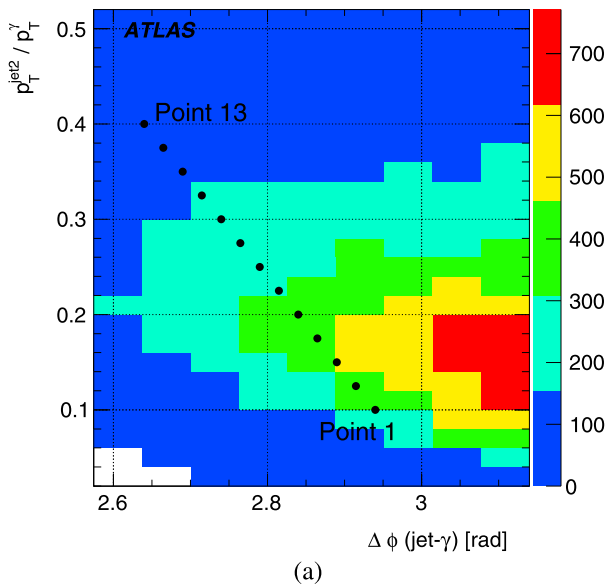
Fig. 28 The values of radiation-suppressing cut thresholds (points) used to probe the soft QCD radiation systematic uncertainty, as a function of \Delta\phi_{jet-\gamma} and p_T^{jet}/p_T^\gamma overlaid with the number of events observed in data (a). The nominal selection is the bottom-rightmost point labelled “Point 1”. Relative change in the MPF re-
