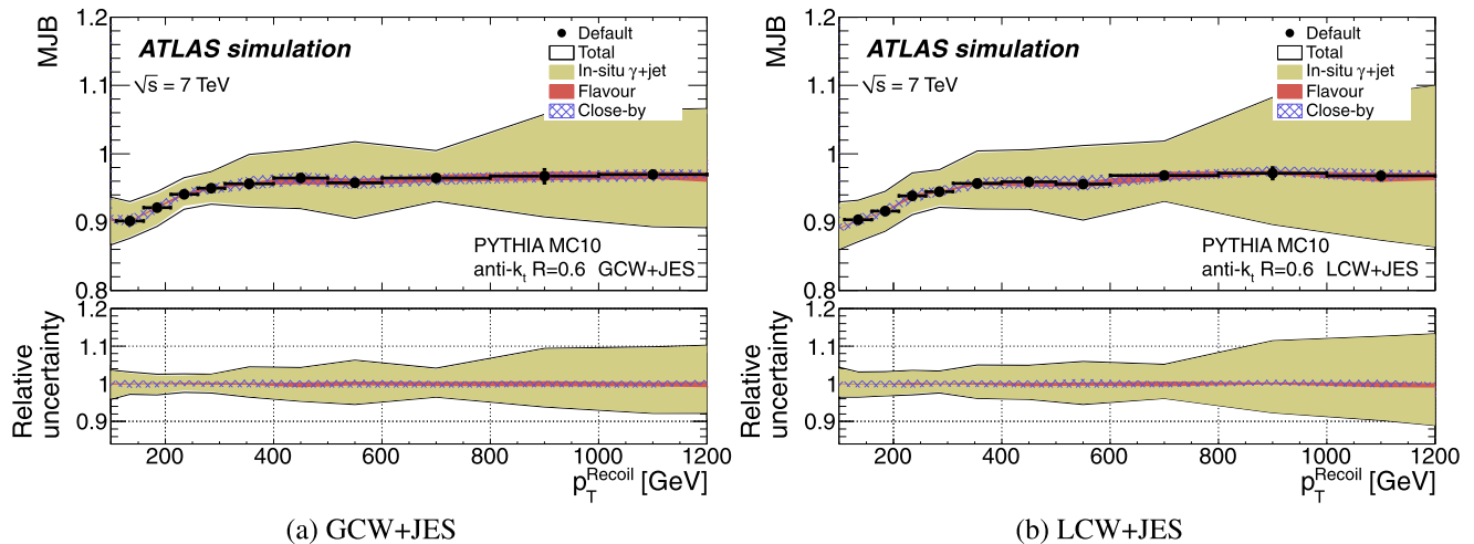
Fig. 67 The multijet balance MJB_{\text{MC}} as a function of the recoil system p_T (full dots) for anti- k_r jets with R = 0.6 using the GCW+JES (a) and LCW+JES (b) calibration schemes. The three bands are defined by the maximum shift of MJB when the jets that compose the recoil system are shifted up and down by the JES uncertainty determined from the \gamma -jet balance, close-by jet and flavour uncertainties. The black
