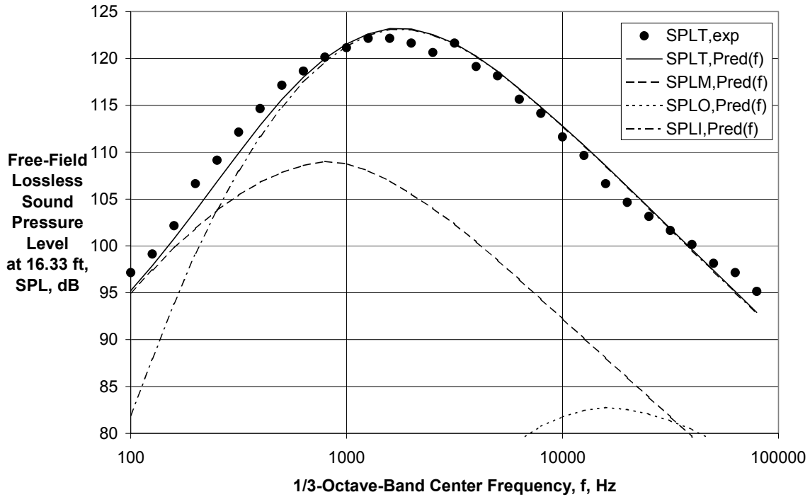
Figure 31 (Concluded) - Comparison of Experimental and First Gen. Pred. Spectra for V_{mix}/C_{amb} = 0.938 , M_f = 0.0 ( A_0/A_1 = 1.94 , Ref. 25, Rdg. 05)
