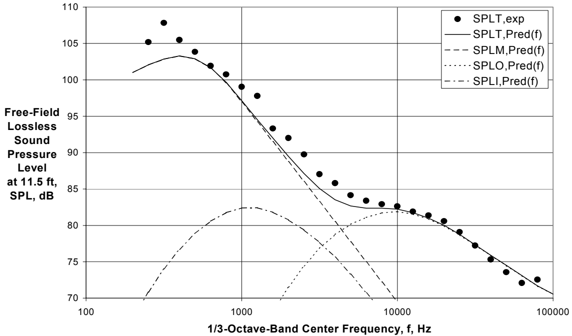
Figure 76 (Concluded) - Comparison of Experimental and Final Predicted Spectra for Internal Plug Nozzle with V_{mix}/c_{amb} = 0.809 , M_f = 0.10 ( A_0/A_1 = 2.72 , Cond. 50010, Ref. 31)
