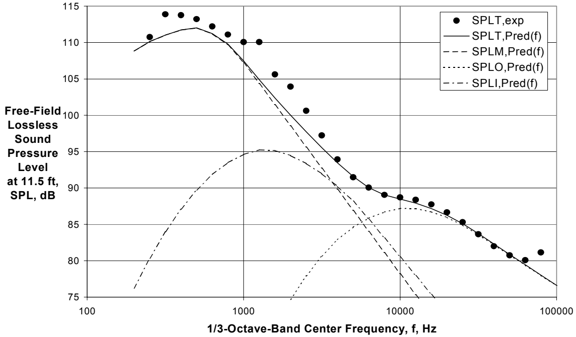
Figure 78 (Concluded) - Comparison of Experimental and Final Predicted Spectra for Internal Plug Nozzle with V_{mix}/c_{amb} = 0.967 , M_f = 0.10 ( A_0/A_1 = 2.72 , Cond. 150010, Ref. 31)
