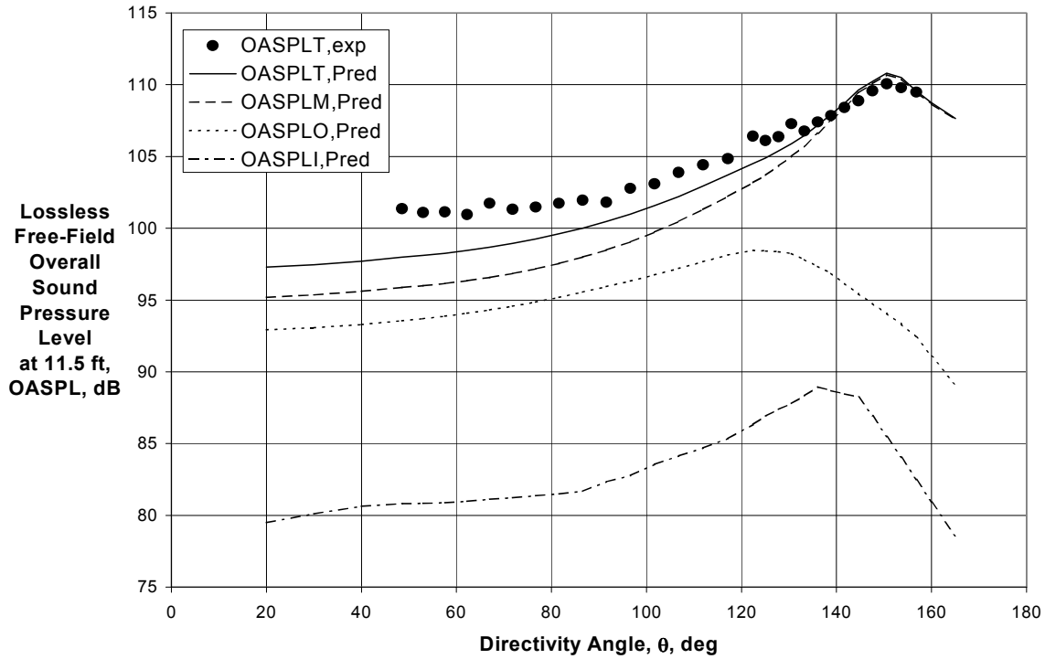
Figure 89 - Comparison of Experimental and Final Predicted Directivities for Internal Plug Nozzle with V_{mix}/c_{amb} = 0.800 , M_f = 0.10 ( A_0/A_1 = 5.66 , Cond. 530010, Ref. 31)
