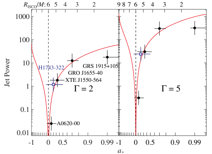
Figure 1. Relationship between radio jet power and the observable R_{\text{ISCO}}/M (top axis) and black hole spin (bottom axis). The value a_* = 0 is marked by a vertical dashed line. The NM12 data are plotted as filled circles and the data for H1743 as an open square. The uncertainty in jet power is uniformly assumed to be a factor of two.
