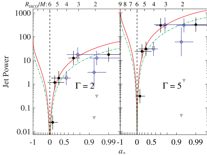
Figure 3. Fe-line spin measurements (open symbols) are compared against the best-fitting NM12 model—the solid curve—which is based on continuum-fitting spin measurements and a fit to the five calibration sources (filled circles) shown both here and in Figure 1. A dot-dashed curve shows the best fit achieved to the Fe-line and continuum-fitting measurements together. Both sets of fits have been computed by assuming that all jets are produced with either \Gamma = 2 (left panel) or \Gamma = 5 (right panel). The jet powers obtained using the fitted inclinations returned by the Fe-line fits are plotted as filled gray triangles.
