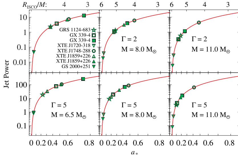
Figure 2. In successive panels, we plot the spin for each black hole listed in Table 1 that results from adopting a value of M ( 6.5 M_{\odot} , 8 M_{\odot} , and 11 M_{\odot} , from left to right) and a value of \Gamma (2 in the upper row and 5 in the lower). The red line in each panel is a fit to the NM12 model using the data for all five calibration sources (Section 3). In producing this figure, we fixed M_2 = 0.3 M_{\odot} for the four systems with measured values of the mass function and arbitrarily show results using i = 60^{\circ} for the two without.
