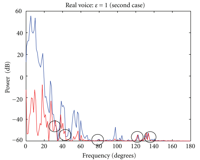
FIGURE 5: Power spectrum of harmonic and subharmonic parts of a real voice. The jitter measured on the time signal was 1 sample but the STJE algorithm counted 5 crossings.
