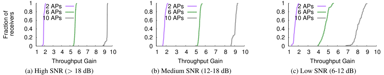
Figure 10: Fairness. CDFs of per-client throughput gain. Across all SNRs, JMB provides all clients with very similar gains.
