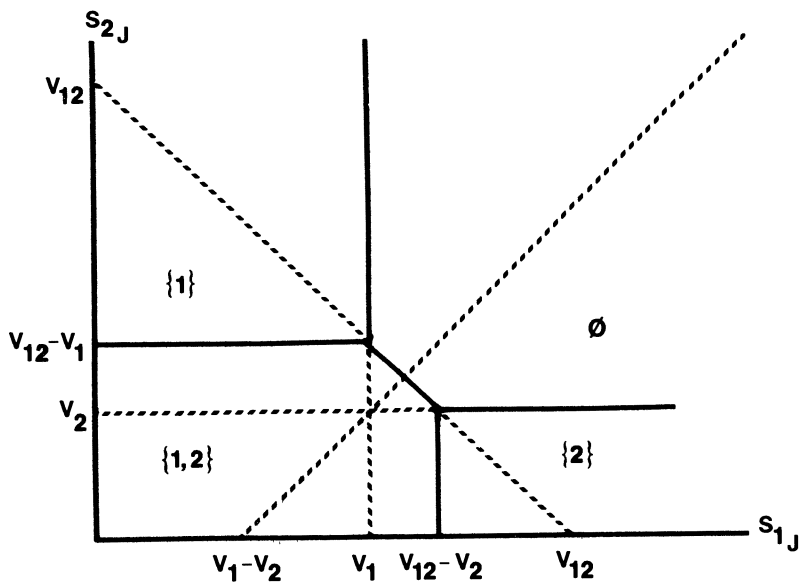
FIGURE 2—Superadditive case.
