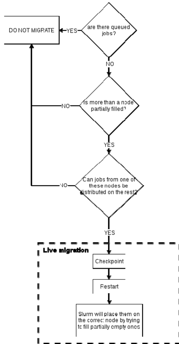
Algorithm 1: Job Compaction scheduling algorithm
