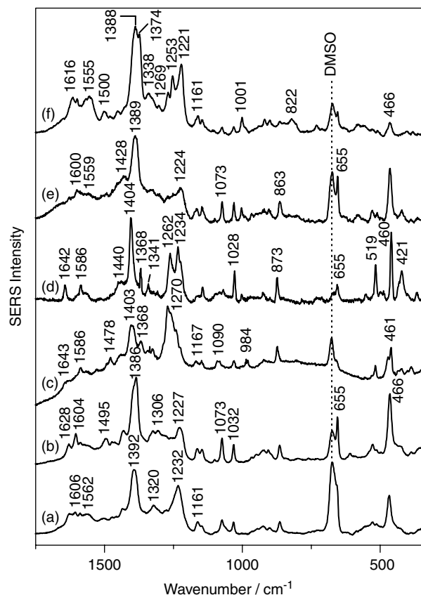
Figure 4. Micro-SERS spectra of QZ ( 10^{-5} M) at pH (a), 11.5 (b) 6.5 and (c) 3.5 and SERS spectra of the following complexes: (d) QZ–HSA; (e) QZ–BSA f ; and (f) QZ–HSA f . All complexes at a 1 : 4 concentration ratio ( 10^{-5} : 4 \times 10^{-5} M).
