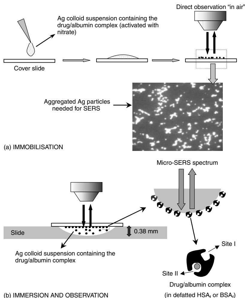
Figure 2. Experimental set-up for micro-SERS measurements.
