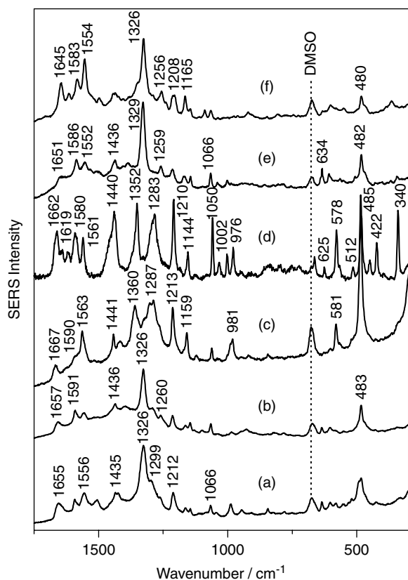
Figure 3. Micro-SERS spectra of DT ( 10^{-5} M) at pH (a), 11.5 (b) 6.5 and (c) 3.5 and SERS spectra of the following complexes: (d) DT–HSA; (e) DT–BSA f ; and (f) DT–HSA f . All complexes at a 1 : 4 concentration ratio ( 10^{-5} : 4 \times 10^{-5} M).
