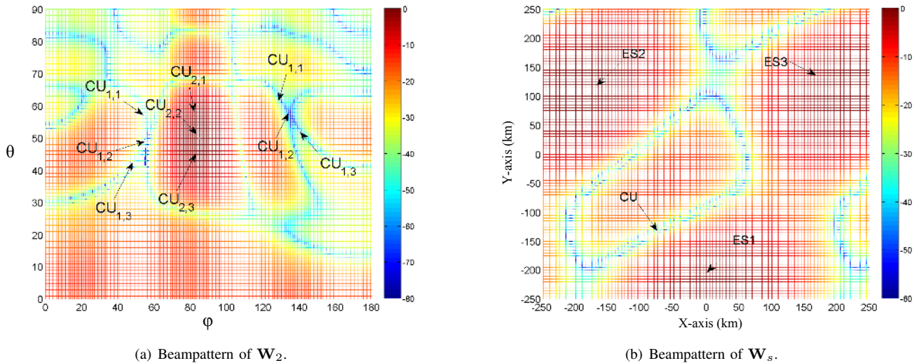
Fig. 5: Beampattern of beamforming weight vectors at BS and SAT.
