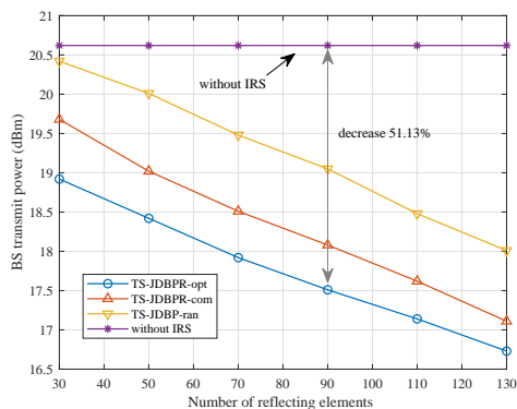
Fig. 8. The BS transmit power versus number of reflecting elements M .
